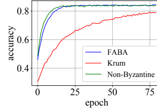
Figure 4: Accuracy
