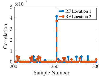
(b) Scenario 2 shows the synchronous reception from two different boards, synced using PPS signal.
