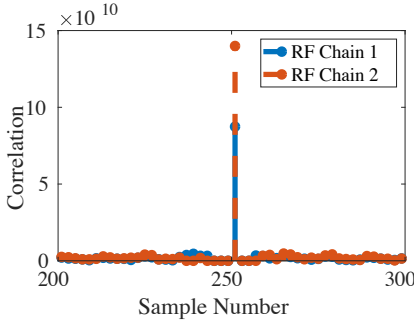
(a) Scenario 1 shows synchronous reception from two RF chains in the same board.
