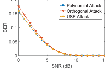
Fig. 10: Decoding BER under different received SNR levels.
