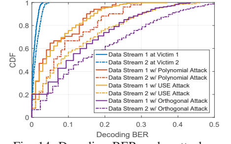
Fig. 14: Decoding BER under attacks.
