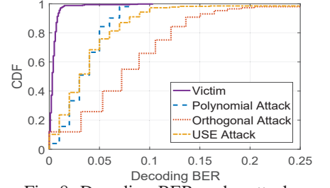
Fig. 8: Decoding BER under attack.
