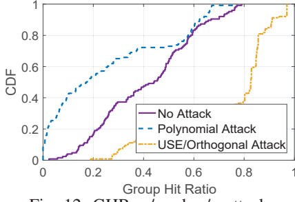
Fig. 12: GHR w/ and w/o attacks.
