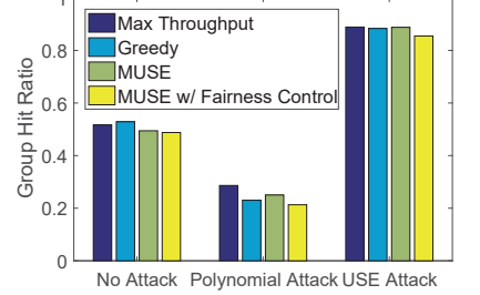
Fig. 11: GHR under different user selection algorithms.
