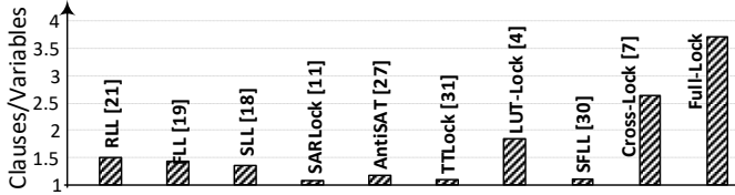
Figure 7: Average Clauses to Variables Ratio for Different Logic Locking Schemes.
