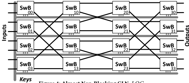
Figure 4: Almost Non-Blocking CLN, LOG_{8,1,1} .
