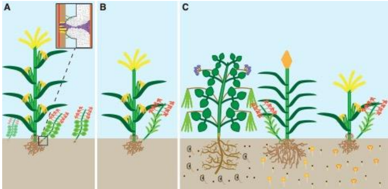
Figure 1. Three-phase model of parasitic plant evolution. (A) Phase I: Facultative parasitism evolves through gain of haustorium development. Inset (adapted from [1]): Haustorial hairs (green) establish contact with host root. Intrusive cells (yellow) penetrate host tissue until they reach host vasculature (red), where some will differentiate into xylem cells (purple) and carry resources back to the parasitic vasculature (orange). (B) Phase II: Evolution toward greater, possibly obligate reliance on host plants through genetic degradation of mechanisms necessary for independent acquisition of resources (e.g. by reducing allocation to leaves). (C) Phase III: Evolution of greater host specificity, for instance through increased selectivity of host-induced germination responses.
