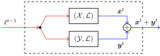
Figure 8. Regret circuit for the Minkowski sum \mathcal{X} + \mathcal{Y} (Section 4.2).
