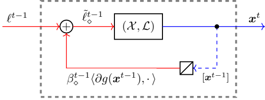
Figure 9. Regret circuit for the Lagrangian relaxation construction (Section 6.1) for the constrained set \mathcal{X} \cap \{x : g(x) \leq 0\} .
