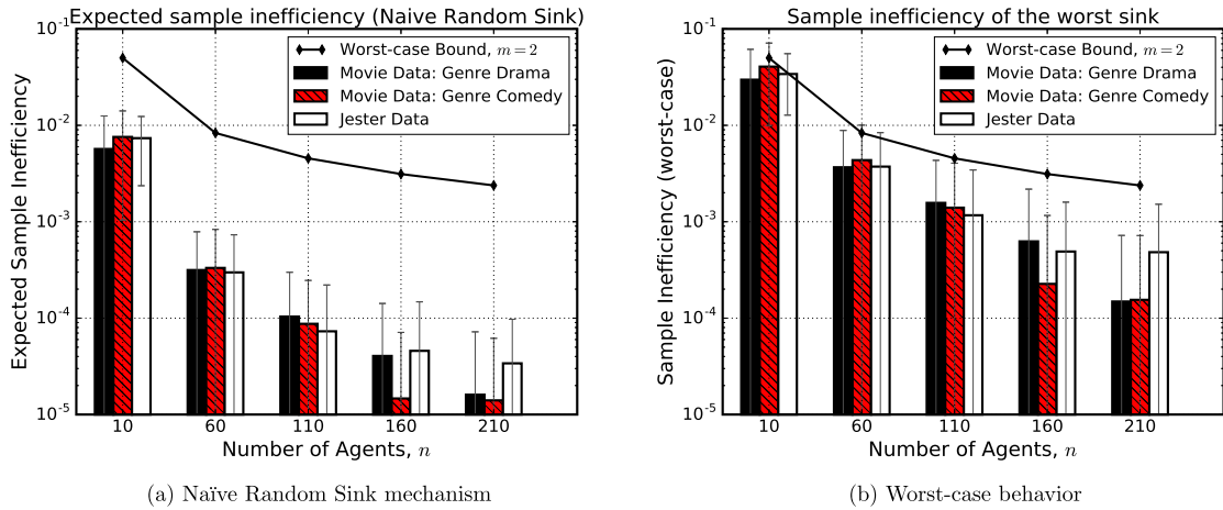
Fig. 2. Performance of naïve randomized sink mechanism on MovieLens and Jester datasets.
