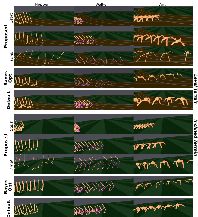
Fig. 1. Our algorithm learns a robot’s physical design jointly with the control policy to optimize performance for a given task and environment. It maintains a distribution over designs, and optimizes a neural network control policy to maximize expected reward over this design distribution using reinforcement learning. The control network has access to the design parameters, allowing it to tailor its policy to each design in the distribution. We shift this distribution towards higher performing designs throughout training, eventually converging to a design and control policy that are jointly optimal. Here, we visualize the evolution of modes of the design distribution and the corresponding learned control policy (gait) for three robot morphologies tasked with locomoting over level (top) and inclined (bottom) terrains. We also show the default Roboschool designs and those learned using Bayesian optimization, along with their learned gaits. Images represent motion with snapshots at fixed time intervals, so designs appearing farther to the right represent faster motion.
