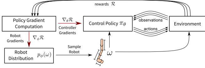
Fig. 2. Overview of our approach. Our proposed algorithm maintains a distribution p_\phi(\omega) over possible physical design parameters. At each iteration of training, a specific design \omega is sampled from this distribution, and an episode is run with that design and the current control policy \pi_\theta in the environment. The policy \pi_\theta has access to the parameters \omega of the robot instance it is controlling in that episode, along with observations fed back from the environment. Policy gradients with respect to episode rewards are then used to update parameters \theta and \phi of both the control policy and the robot distribution, respectively.
