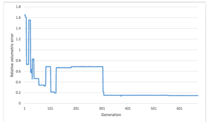
Fig. 13. The relative volumetric error of the elite CSG tree in the genetic algorithm's population, vs. generation. The energy in [Fayolle and Pasko 2016] is purely defined on the surface difference so it fails to capture the volumetric change. Thus, while energy monotonically increases, the volumetric error oscillates between generations.
