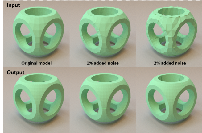
Fig. 16. Solving input meshes with different amount of noises. Top row from left to right: 0, 1, and 2 noises are added. Bottom row: our solutions.
