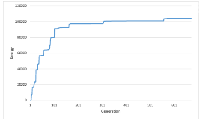
Fig. 12. The energy as defined by [Fayolle and Pasko 2016] of the elite CSG tree in the genetic algorithm's population, vs. generation. While the energy improves rapidly at the beginning, it is unable to resolve all discrepancies between the input and generated mesh after 672 iterations.
