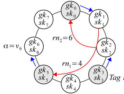
Fig. 3. Key Issuing.
