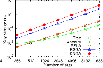
Fig. 10. The key storage cost.
