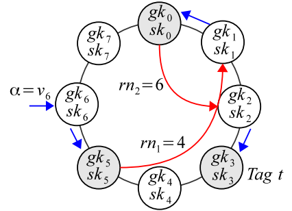
Fig. 4. Authentication.
