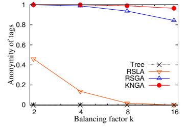
Fig. 8. Anonymity with n_c = 2048 .
