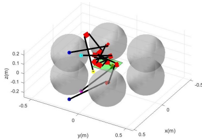
Fig. 9: Solution returned for Problem 1 with n_{\text{obs}} = 6 , n_{\text{task}} = 5 , and, n_{\text{mod}} = 3 . The blue dots are the original task, the others are additional user inputs.
