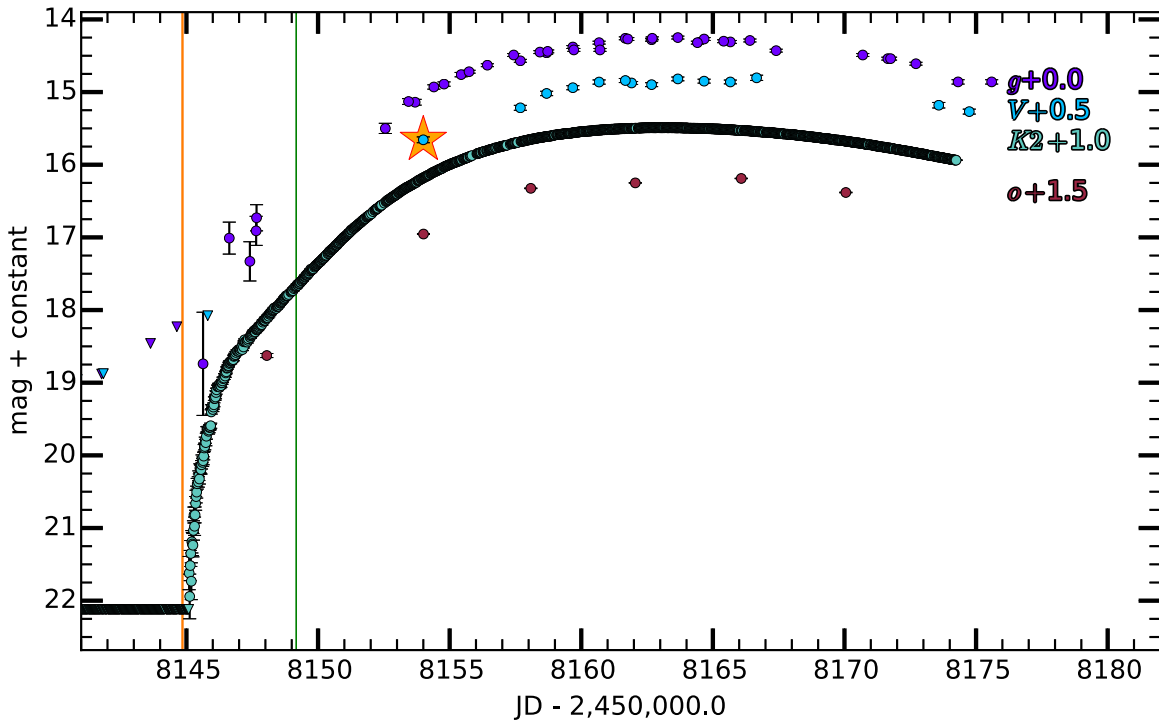
Figure 2. Host-subtracted light curves of ASASSN-18bt from ASAS-SN (V and g filters), K2 ( Kepler filter), and ATLAS (“orange” or o filter). Here, 3\sigma limits are shown as downward triangles for epochs where the supernova was not detected. The orange and green vertical bars indicate t_1 and t_2 , respectively, as determined by a double-power-law fit to the K2 light curve (see Section 3 and Equation (1)). The orange star highlights the ASAS-SN discovery epoch of ASASSN-18bt.
