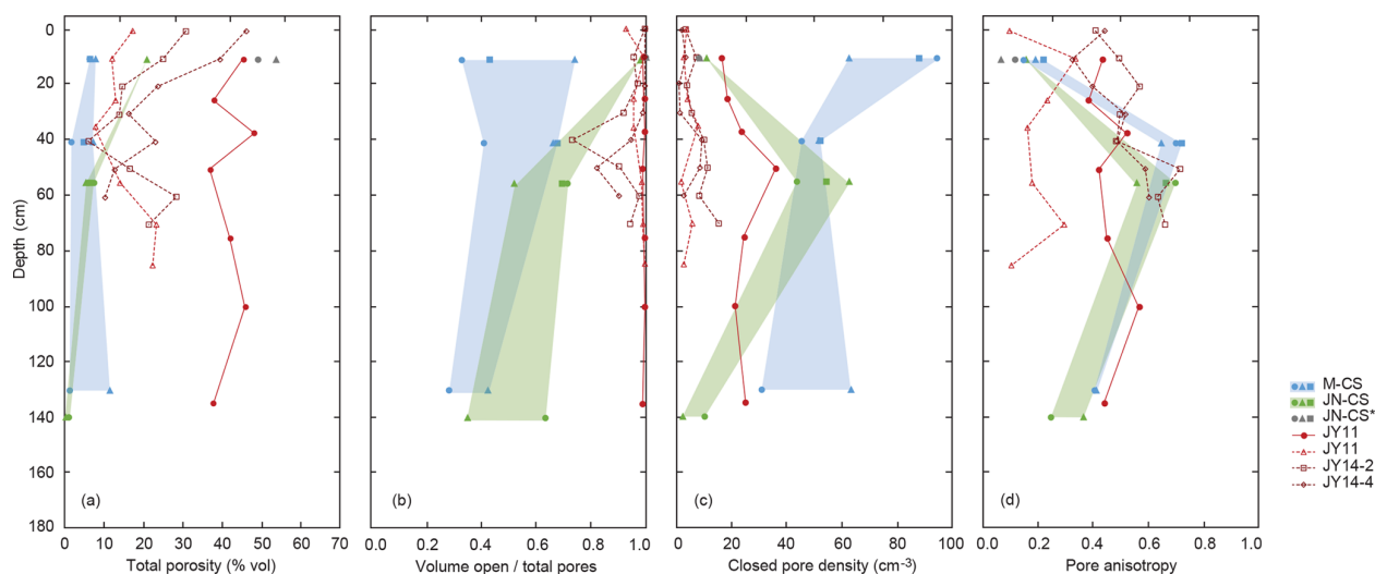
Figure 10. Sea ice internal pore properties calculated from 3-D reconstructions of micro-CT scans of cuts of cores collected in May, June, and July. (a) Total porosity as a percentage of the analyzed volume. (b) Volume of open pores vs. total volume of pores in the analyzed volume. (c) Average spatial density of closed pores in the analyzed volume. (d) Anisotropy of pores in the analyzed volume. Depths indicate the in situ depth within the ice of the top of the volume of interest used for the calculations. Colors indicate sampling month: May (M-CS; blue), June (JN-CS; green), and July (JY11 and JY14 in red and dark red, respectively). Shaded blue and green fields represent the range of values measured in replicate ice horizon samples in May and June, respectively. Closed markers indicate DMP-casted samples; open markers indicate non-casted samples. Values calculated from a volume believed to be representative of a retextured snow layer in the uppermost June samples are represented by gray symbols. For all points, the volume analyzed was a 77.6 \text{ cm}^3 cylinder (diameter = 4.97 cm, height = 4.0 cm) selected from a representative portion of the interior of the cut sea ice horizon.
