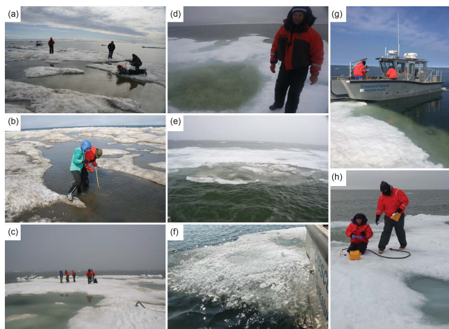
Figure 3. Photographs of specific rotten ice sampling sites in July: (a) JY3-L3, (b) JY10, (c) JY11, (d) JY14-L3, (e) JY14-L4, (f) JY13-L1, (g) JY13-L2, (h) JY17-L1.
