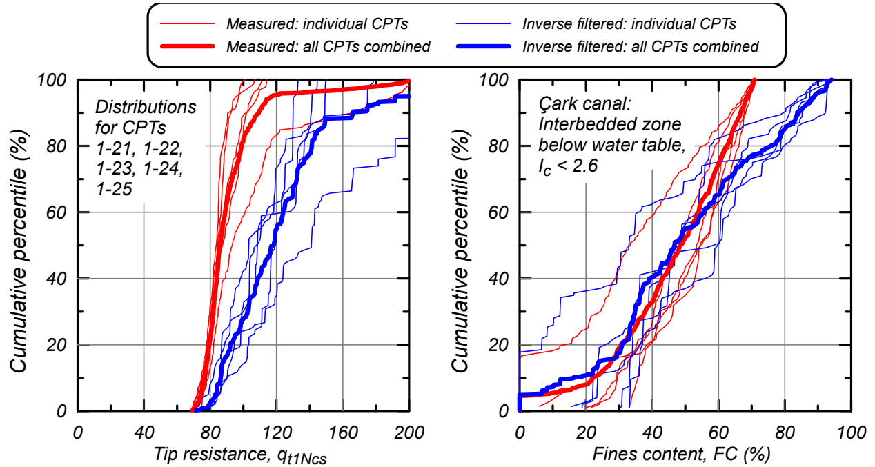
Figure 8. Cumulative distributions of equivalent clean sand, overburden-corrected tip resistance and fines content for the sand-like soils within the interbedded stratum beneath the water table for the measured CPT data (red lines) and inverse filtered data (blue lines)
