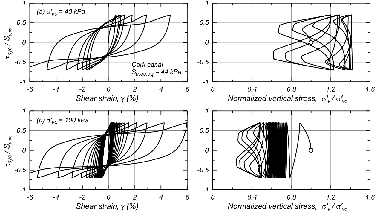
Figure 15. Cyclic stress-strain responses for the clay-like soils at two overburden stresses from single element simulations of undrained DSS loading with PM4Silt
