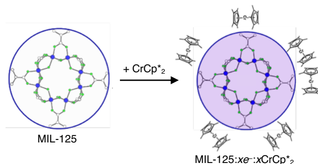
Figure 1: Reduction of MIL-125 with CrCp* 2 .
