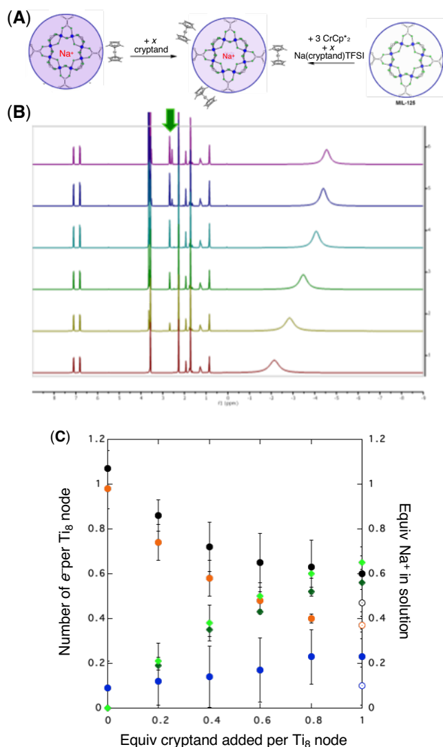
Figure 4: Effect of adding cryptand to reduced MIL-125 (3 equiv \text{CrCp}^{*2} + 1 equiv of \text{Na}^+ ), and reduction of MIL-125 with \text{CrCp}^{*2} and (\text{Na}\cdot\text{cryptand})\text{TFSI} . (A): Schematic of this reaction. (B): ^1\text{H} NMR spectra ( d_8 -THF+ \text{CD}_3\text{CN} , 4:1 v/v) MIL-125 + 3 equiv \text{CrCp}^{*2} + 3 equiv \text{NaTFSI} + 0 (red), 0.2 (yellow), 0.4 (green), 0.6 (light blue), 0.8 (dark blue), and 1.0 (purple) equiv cryptand (per \text{Ti}_8 node). The two peaks indicated by the arrow correspond to free (right) and Na-bound (left) cryptand. (C): Plot of e^- in MIL-125 versus equivs of cryptand added (left axis), and equiv of \text{Na}^+ in solution (right axis). Orange circles: equivs \text{Na}^+ associated with the reduced MIL-125, derived from the \text{CrCp}^{*2/0+} chemical shift. Blue circles: equivs \text{CrCp}^{*2} associated with the reduced MIL-125, derived from the change in integration of the \text{CrCp}^{*2/0+} resonance. Black circles: total extent of reduction (sum of blue and orange). Light green diamonds: equiv \text{Na}^+ in solution, derived from the amount of \text{Na}^+ still associated with reduced MIL-125. Dark green diamonds: equiv of \text{Na}^+ in solution, from integration of the cryptand/cryptand-sodium resonances. Open circles: number of e^- in MIL-125 (per \text{Ti}_8 node) for the converse reaction: addition of 3 equiv of \text{CrCp}^{*2} and 1 equiv of \text{Na}^+(\text{cryptand})\text{TFSI}^- .
