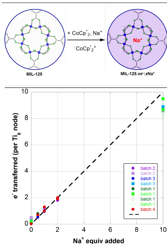
Figure 5. (Top): Schematic of the reduction of MIL-125 with \text{CoCp}^*_2 . The darkening indicates addition of electrons, and incorporation of sodium is designated by the red \text{Na}^+ . (Bottom): Extent of MIL-125 reduction versus equiv of \text{Na}^+ added to various batches of MIL-125. Experiments with 2 (circles) and 10 (squares) equiv of \text{CoCp}^*_2 are plotted. The dashed line represents a 1:1 stoichiometry, and is not a fit. Description of the MIL-125 crystallites are: batch 1 has ellipsoid morphology and axes of 300 (\pm 100) - 850 (\pm 50) nm; batch 2 has spherical morphology with axes of 85 (\pm 17) nm; batch 3 has octahedral morphology with edges of 2650 (\pm 1350) nm; batch 4 contains deuterated bdc linkers and has ellipsoid morphology and axes of 600 (\pm 200) - 1150 (\pm 350) nm.
