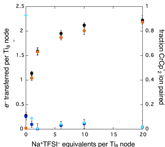
Figure 3: Reduction of MIL-125 with 6 equiv CrCp* 2 and 0-20 equiv Na + in ds -THF+CD 3 CN 4:1 v/v). Plot of e - transferred to MIL-125 (left axis), and fraction of CrCp* 2 ion-paired in reduced MIL-125 (right axis), versus equiv NaTFSI added. Orange circles: equiv Na + associated with the reduced MIL-125, derived from the CrCp* 2 0/+ chemical shift. Blue circles: equiv CrCp* 2 + that are associated with the reduced MIL-125, derived from the change in integration of the CrCp* 2 0/+ resonance upon mixing with MIL-125. Black circles: total extent of reduction (sum of blue and orange). Light blue diamonds represent the fraction of the reduced MIL-125 that is associated with CrCp* 2 + .
