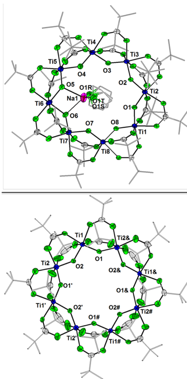
Figure 6. Displacement ellipsoid (50%) representation of (top) 2-Na and (b) the anion of 2-CoCp* 2 . For clarity, H-atoms are omitted and t\text{Bu} groups are shown as sticks. There are two THF ligands to \text{Na}^+ that are disordered, as shown (S: 24.5%, R: 75.5%); see the ESI. Select bond distances (Å) for 2-Na : Ti1-O8 1.7796(25), Ti1-O1 1.8090(24), Ti2-O1 1.8090(25), Ti2-O2 1.7939(24), Ti3-O2 1.8285(24), Ti3-O3 1.7660(25), Ti4-O3 1.8634(25), Ti4-O4 1.7456(27), Ti5-O4 1.9075(26), Ti5-O5 1.7451(28), Ti6-O5 1.9473(27), Ti6-O6 1.9556(26), Ti7-O6 1.7346(27), Ti7-O7 1.8830(26), Ti8-O7 1.7571(25), Ti8-O8 1.8459(25). Select bond distances (Å) for 2-CoCp* 2 : Ti1-O2 1.8445(1), Ti1-O1 1.7990(1), Ti2-O1' 1.8514(1), Ti2-O2 1.7666(1).
