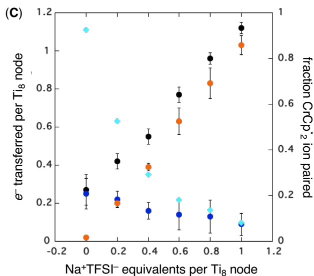
Figure 2: Reduction of MIL-125 with CrCp ^*_2 and Na ^+ (NaTFSI). (A): Schematic of the reaction. (B): ^1\text{H} NMR spectra ( d_8 -THF+CD _3 CN 4:1 v/v) of mixtures of MIL-125 + 3 equiv CrCp ^*_2 + different equiv of Na ^+ per Ti _8 node: 0 (red), 0.2 Na ^+ (yellow), 0.4 Na ^+ (green), 0.6 Na ^+ (light blue), 0.8 Na ^+ (dark blue), and 1.0 Na ^+ (purple). (C): Plot of e^- transferred to MIL-125 (left axis) and fraction of CrCp ^*_2 ion-paired in reduced MIL-125 (right axis) versus equiv NaTFSI added. Orange circles: equiv of Na ^+ associated with the reduced MIL-125, derived from the CrCp ^*_2 ^{0/+} chemical shift. Blue circles: equiv CrCp ^*_2 ^+ associated with the reduced MIL-125, derived from the change in integration of the CrCp ^*_2 ^{0/+} resonance upon mixing with MIL-125. Black circles: total extent of reduction (the sum of the blue and orange circles). Light blue diamonds: fraction of the reduced MIL-125 that is associated with CrCp ^*_2 ^+ .
