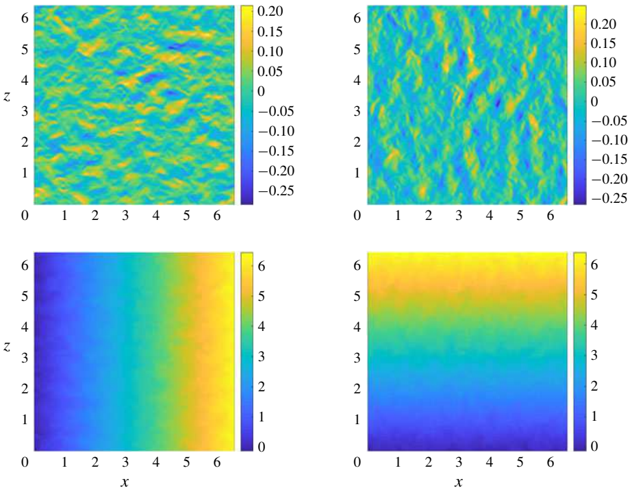
FIGURE 19. Snapshots of u , w , x+v and z+\theta at time t=100 for the case with l_o \ll l_f .
