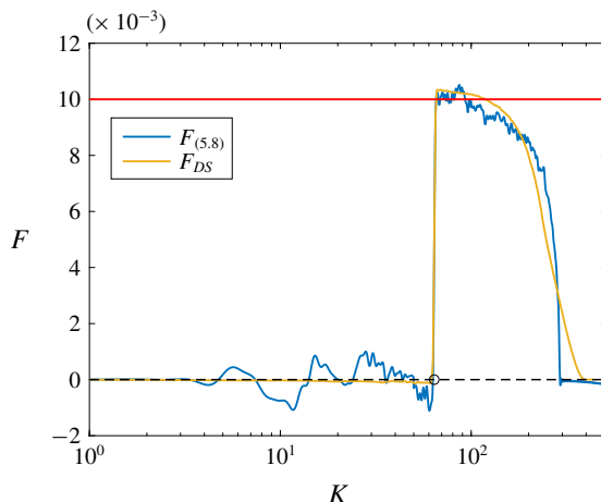
FIGURE 11. Comparison between the spectral total energy flux recovered from the structure function V using (5.8) F_{(5.8)} and that obtained from direct statistics F_{DS} in the strong forcing regime. The red line marks the level of \epsilon = 0.01 , the circle marks the forcing scale and the black dashed line is the 0-line for reference.
