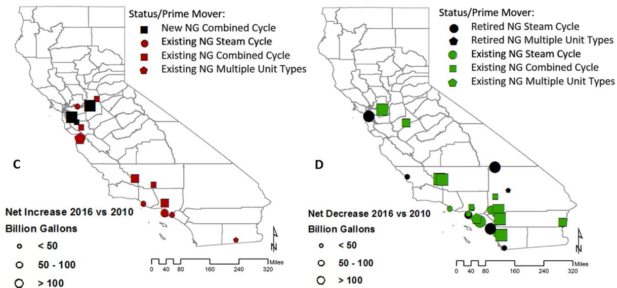
Fig. 3. Net changes in CO 2 emissions (increase in A, decrease in B) and cooling water consumption (increase in C and decrease in D) across California's natural gas electricity generation fleet in 2016 versus 2010. Each shape represents a power plant categorized into five categories, i.e. combined cycle, steam cycle, gas turbine, internal combustion engines and power plants with multi-type prime movers.
