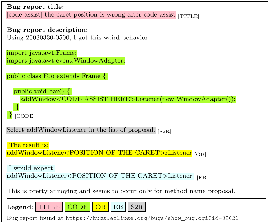
Fig. 1 Bug report #89621 from Eclipse. The highlighted text corresponds to the title (TITLE), code snippets (CODE), observed behavior (OB), expected behavior (EB), and steps to reproduce (S2R)
