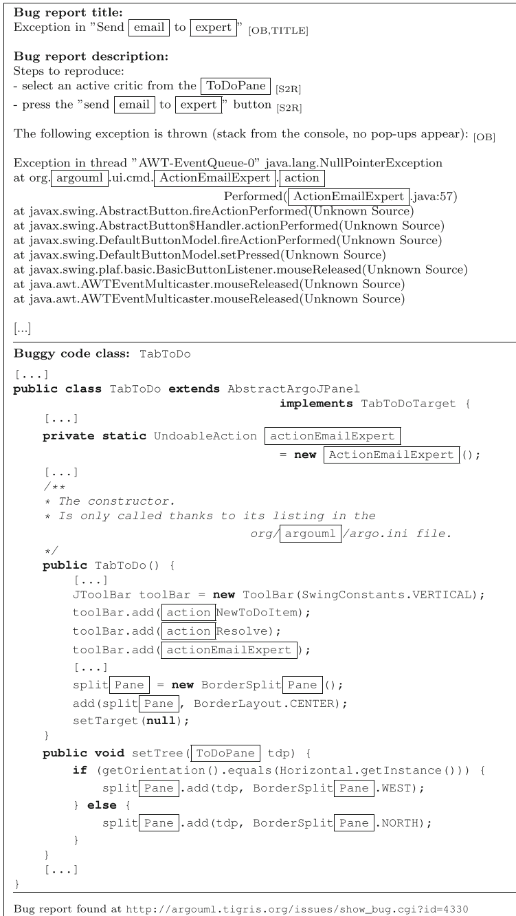
Fig. 4 Bug report #4330 from ArgoUML and its corresponding buggy class. The boxed terms represent the terms shared between the report and the class. Each sentence in the report is marked according to its corresponding information type: [TITLE], [OB], or [S2R]
