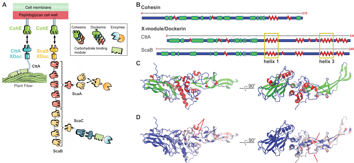
Figure 1: Homology model of ScaB-XDoc:CohE. (A) Schematic of the Rf cellulosome protein network for fiber degradation. 20 The two cell-surface anchoring complexes are CttA-XDoc:CohE and ScaB-XDoc:CohE. (B) Representation of secondary structures of Coh (CohE), and XDoc domains from both CttA (PDB ID: 4IU3) and ScaB (model protein). (C) The structural homology model of the ScaB-XDoc:CohE complex colored by secondary structure and (D) colored by sequence similarity (BLOSUM60) to CttA-XDoc:CohE. In D, regions indicated by red arrows are ScaB-XDoc insert sequences not present in CttA.
