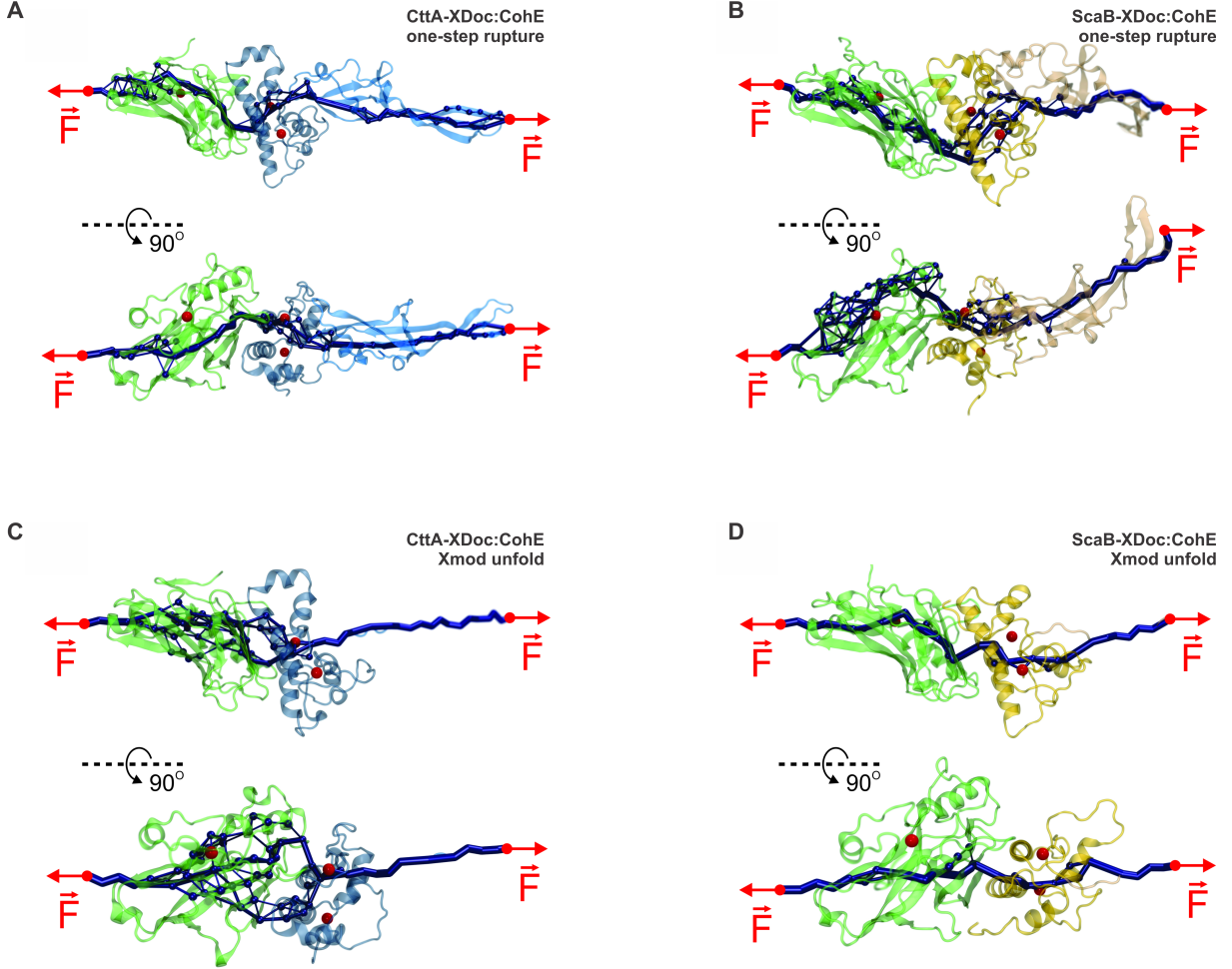
Figure 6: Evolution of force propagation pathways. Force propagation pathways were calculated from correlation-based network analysis carried out using SMD trajectories within 4.0 ns windows just prior to rupture. For one-step rupture of complexes CttA-XDoc:CohE (A) and ScaB-XDoc:CohE (B), force-propagation routes nonparallel to the pulling axis are observed near the Doc:Coh interface. For complex rupture following Xmod unfolding in CttA-XDoc:CohE (C) and ScaB-XDoc:CohE (D) simulation, we again observed redirection of force near XDoc:Coh interface. The thickness of the dark blue tubes represents the number of suboptimal correlation paths connecting two nodes. Thicker tubes correspond to higher likelihood of force propagating through a path. The observed changes in force direction, presented mostly as sharp turns in force propagation routes particularly near the interface, suggest that the ultrastable complexes formed by Coh and Doc achieve mechanostability by directing externally applied forces normal to the pulling axis. Consequently, more force is required to achieve a given separation along the pulling axis.
