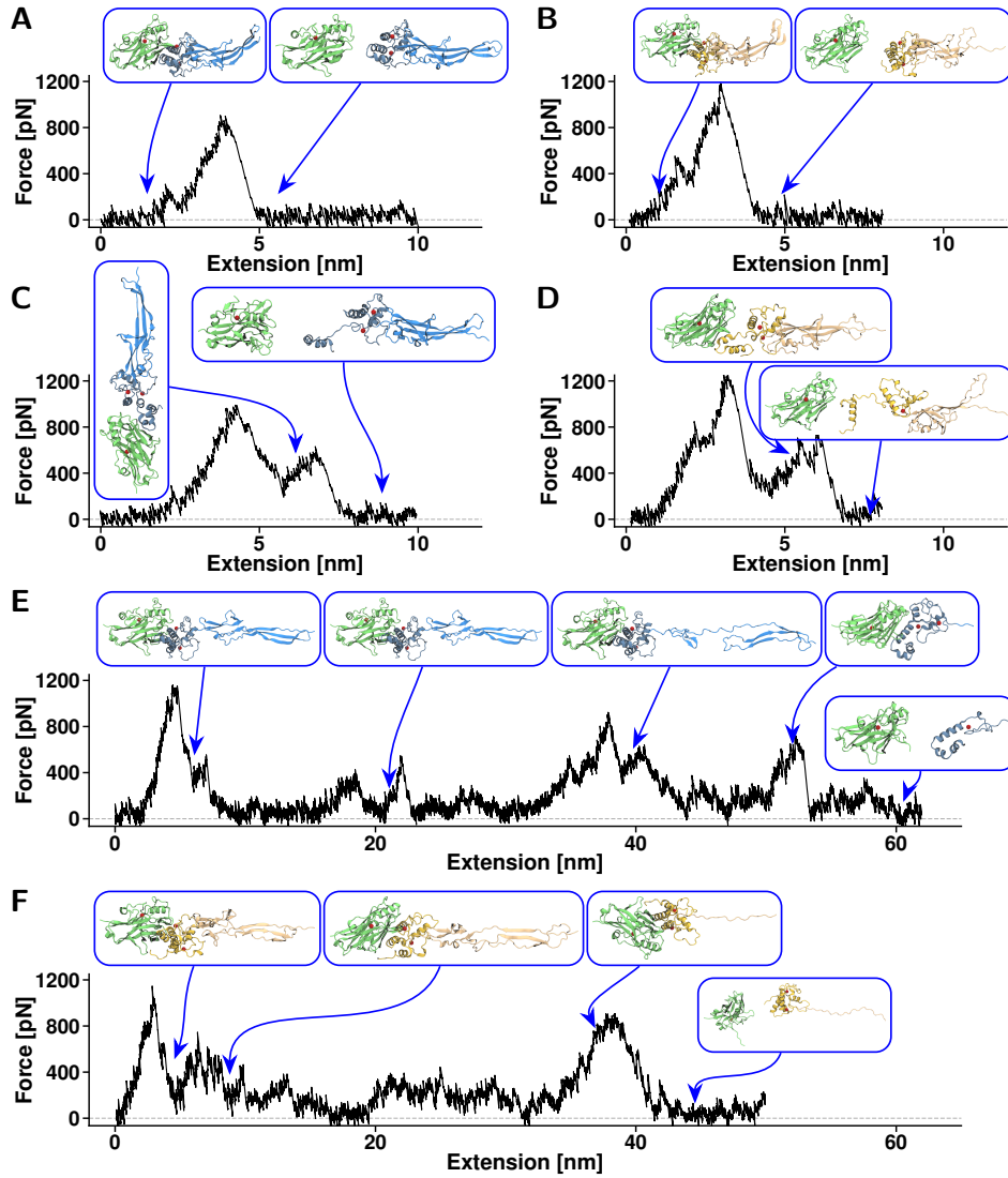
Figure 3: Exemplary force-extension traces from steered molecular dynamics simulations.
