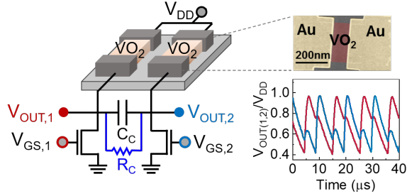
Fig. 3: An IMT device coupled through its Resistive and Capacitive elements showing frequency locking.
