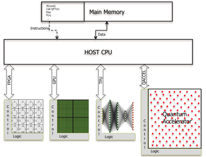
Fig. 1: System architecture with heterogeneous accelerators.
