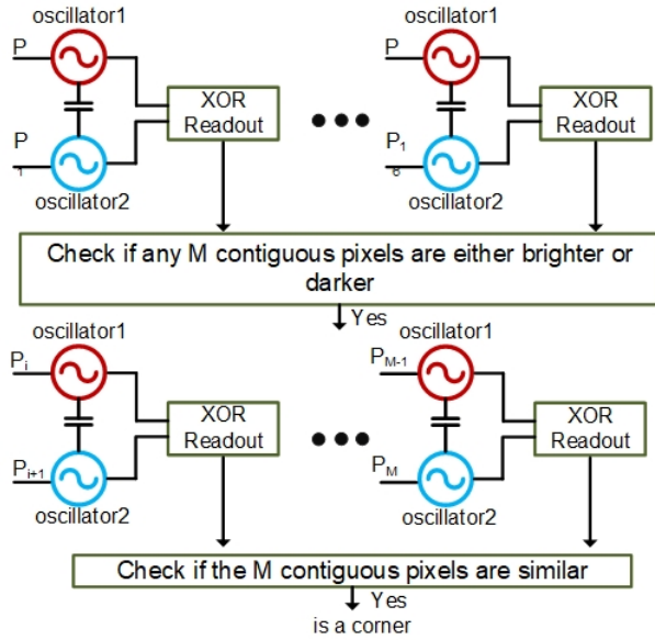
Fig. 6: FAST corner detection using coupled oscillator distance norms.
