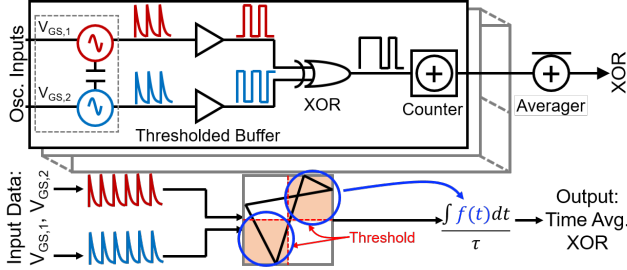
Fig. 4: Readout scheme for pairwise coupled oscillators based on a thresholded and time-averaged XOR.
