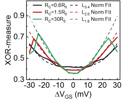
Fig. 5: XOR-measure showing various l_k norms achieved with coupled oscillators.
