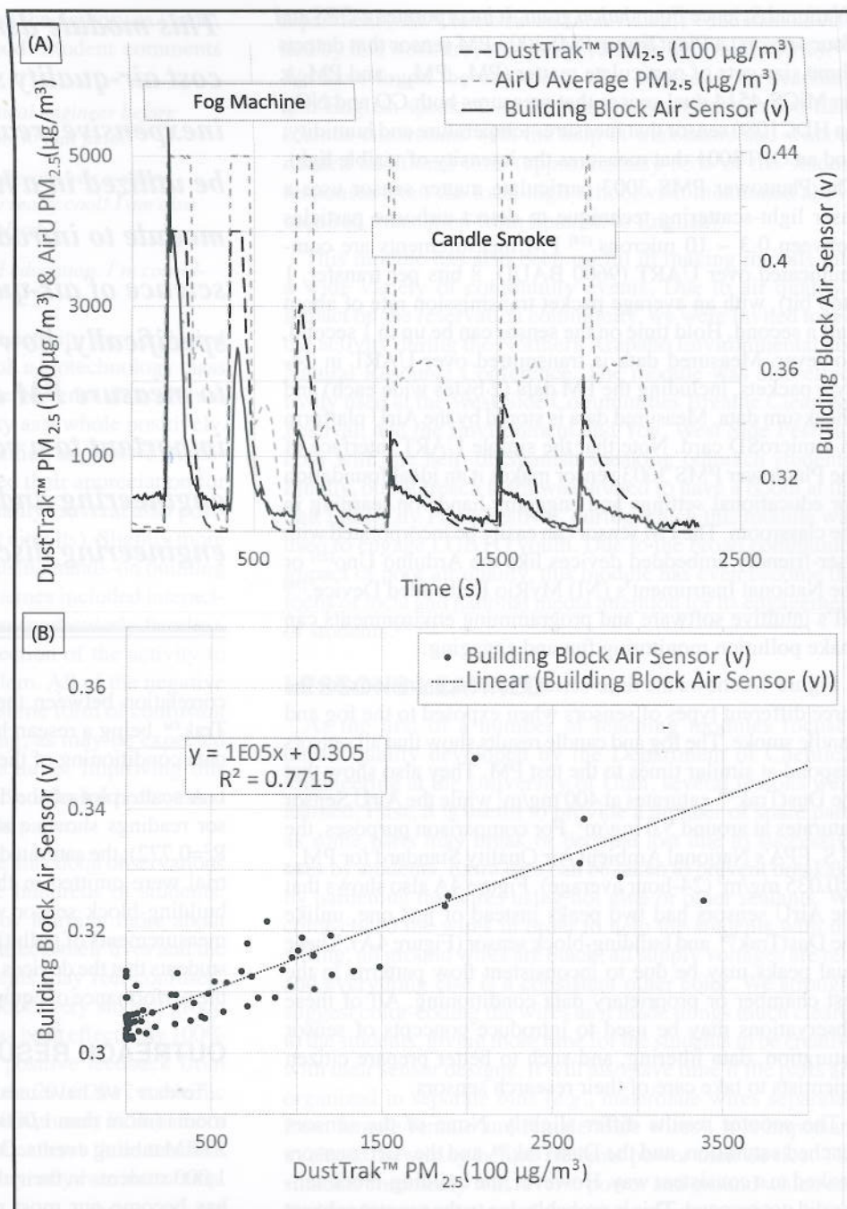
Figure 4. (A) Time series of all sensors' PM measurements during fog and candle trials. Three trials of each were conducted, hence three peaks. (B) Building Block Air Sensor air graphed against DustTrak™ during the fog and candle trial.
