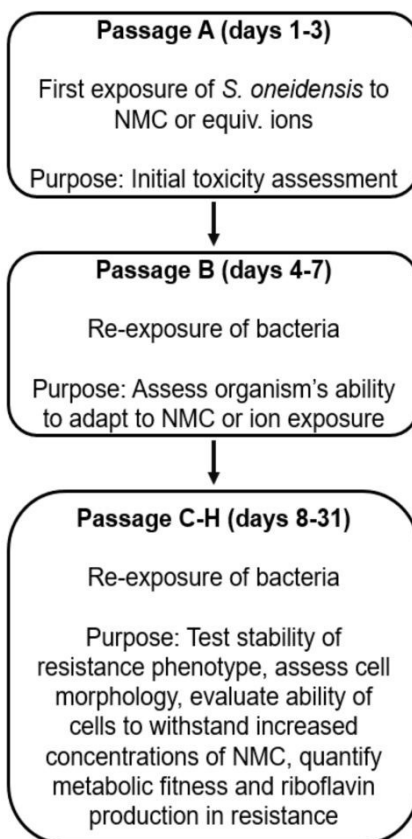
Figure 1. Schematic of experiments performed in this work to assess S. oneidensis MR-1 resistance to NMC. A more detailed schematic is provided in Figure S3 .
