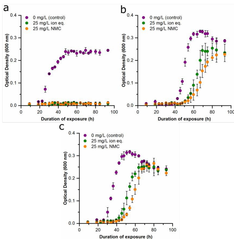
Figure 4. Effect of repetitive NMC and ion exposure on growth inhibition of S. oneidensis MR-1 (Passage C). (a) Bacteria cultured for two passages in pristine media exposed to no NMC (purple), 25 mg/L NMC ion eq. (green), and 25 mg/L NMC (orange). (b) Bacteria cultured for two passages with 25 mg/L NMC, which was then exposed to no NMC (purple), 25 mg/L NMC ion eq. (green), and 25 mg/L NMC (orange). (c) Bacteria cultured for two passages with 25 mg/L NMC ion eq., which was then exposed to no NMC (purple), 25 mg/L NMC ion eq. (green), and 25 mg/L NMC (orange). Error bars represent the standard deviation of three replicates.
