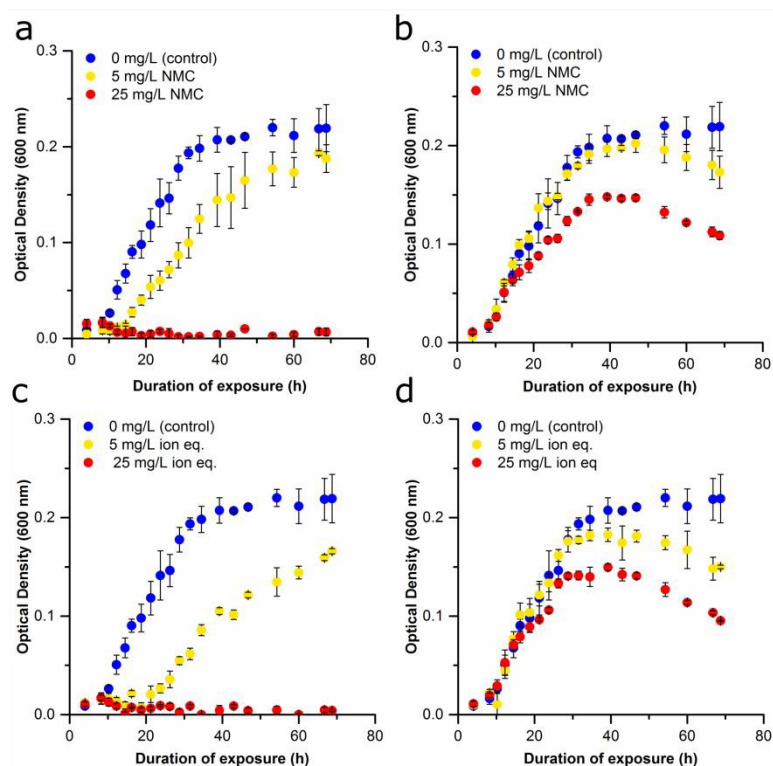
Figure 2. Effect of delayed NMC and ion exposure on growth inhibition of S. oneidensis MR-1 (Passage A). (a) Bacterial exposure at the time of inoculation to no NMC (blue), 5 mg/L NMC (yellow), and 25 mg/L NMC (red). (b) Bacterial exposure 10 h after the inoculation to no NMC (blue), 5 mg/L NMC (yellow), and 25 mg/L NMC (red). (c) Bacterial exposure to constitutive ions of NMC at time of inoculation: no NMC ions (blue), ions of 5 mg/L eq. of NMC (yellow), and ions of 25 mg/L eq. of NMC (red). (d) Bacterial exposure to constitutive ions of NMC 10 h after inoculation: no NMC ions (blue), ions of 5 mg/L eq. of NMC (yellow), and ions of 25 mg/L eq. of NMC (red). Error bars represent the standard deviation of three replicates.
