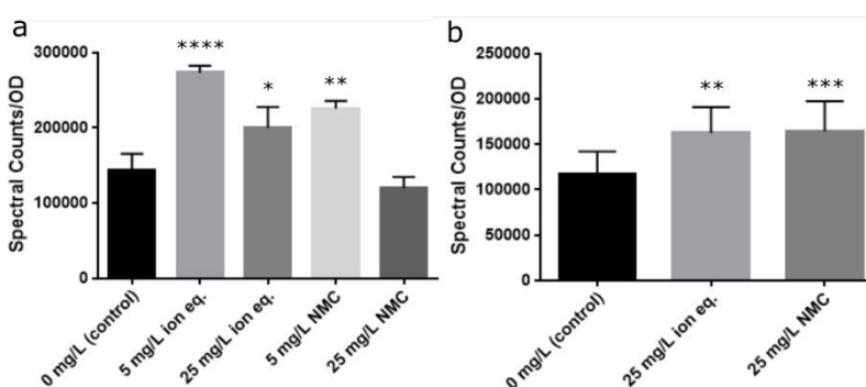
Figure 8. Riboflavin secretion as measured with LC-MS. (a) Passage A demonstrates significant differences between the treated groups and the control. (b) Over multiple subsequent passages (average of B–E), the control differs from the ion- and NMC-treated samples, but these samples do not differ from one another. Statistical analysis performed with non-parametric one-way ANOVA with Tukey analysis as necessary ( \alpha = 0.05 ; **** p \leq 0.0001 ; *** p \leq 0.001 ; ** p \leq 0.01 , * p \leq 0.05 ).
