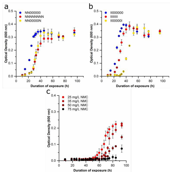
Figure 6. Examination of the stability of the bacterial adaptation following a period of non-exposure (Passage H). (a) Bacteria cultured for two passages in 25 mg/L NMC were then grown for 5 passages without exposure, and then a final passage exposed to 25 mg/L NMC (NN00000N;
