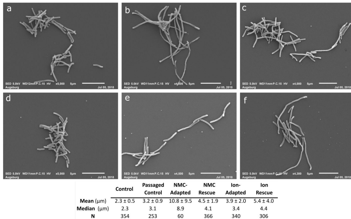
Figure 7. Morphology assessment. Scanning electron micrographs of S. oneidensis MR-1 from Passage D exposed to a) no nanoparticle or ions over 4 passages, b) 25 mg/L NMC over 4 passages c) 25 mg/L NMC ion eq. over 4 passages d) no nanoparticle or ions for one passage, e) 25 mg/L NMC over 2 passages followed by 2 passages without exposure, f) 25 mg/L NMC ion eq. over 2 passages followed by 2 passages without exposure. Table indicates mean, median, and standard deviation in \mu\text{m} for the imaged microbe populations. Statistical analyses to compare the lengths of the bacteria are included in the supporting information ( Figure S12 ).
