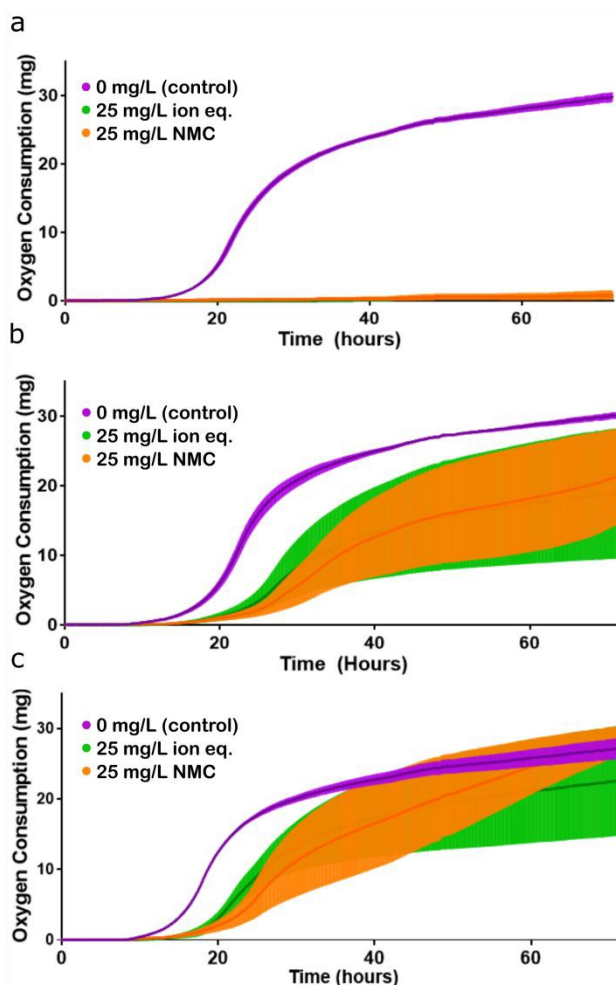
Figure 5. Assessment of organismal fitness by measurement of oxygen consumption. (a) Respirometry curves of S. oneidensis MR-1 control (unadapted) cultures exposed to control conditions (purple), 25 mg/L NMC (orange), and 25 mg/L NMC ion eq. (green) in Passage E. (b) Respirometry curves of NMC-adapted cultures exposed to control conditions (purple), 25 mg/L NMC (orange), and 25 mg/L NMC ion eq. (green) in Passage E. (c) Respirometry curves of ion-adapted cultures exposed to control conditions (purple), 25 mg/L NMC (orange), and 25 mg/L NMC ion eq. (green) in Passage E. Error bars represent the standard deviation of replicates. Representation of Figure 5 without standard deviations is located in Figure S7.
