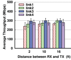
(c) Throughput of each link (downlink) at different distances when 4 links operate concurrently
