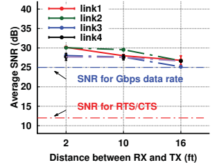
(d) SNR of each link (downlink) at different distances when 4 links operate concurrently
