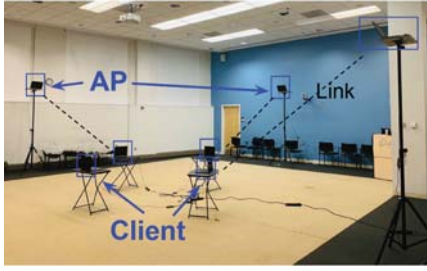
Fig. 3: Setup of 4 links in a 36ft×36ft classroom
