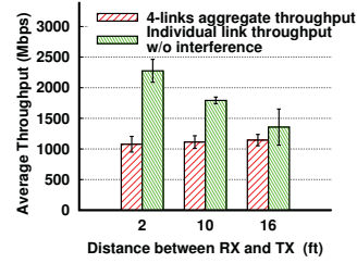
(b) Aggregate throughput of 4 links vs. individual throughput at different distances
