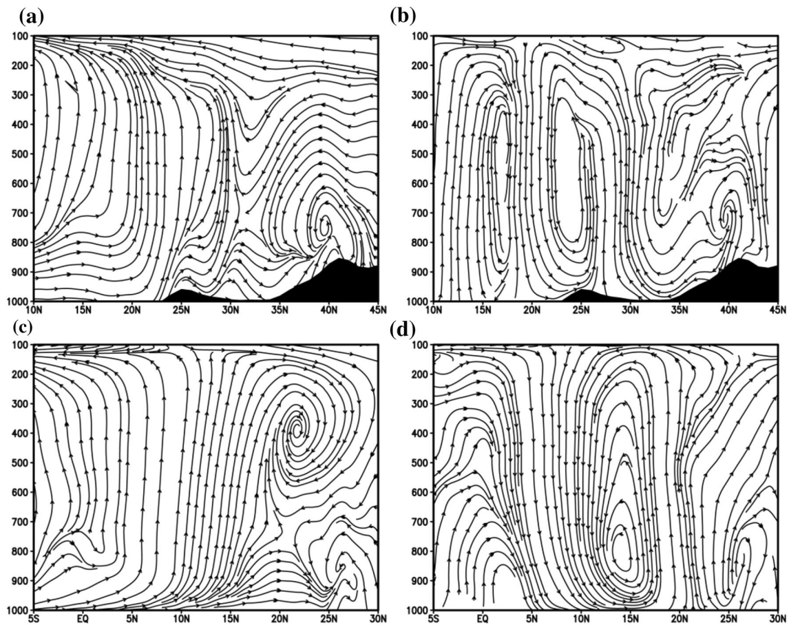
Fig. 6 JJA latitude-height cross section of (a, c) streamline ( v ; -w \times 100 ) in CTL1 and (b, d) differences between ICE and CTL1 (ICE-CTL1) averaged over 105°E–130°E (upper panel) and over 60°E–70°E (bottom panel)
