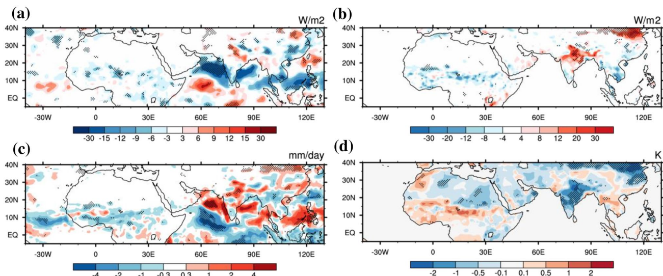
Fig. 5 JJA differences of a surface net radiation ( \text{W/m}^2 ), b latent heat ( \text{W/m}^2 ), c precipitation ( \text{mm/day} ), and d surface temperature (K) between ICE and CTL1 (ICE-CTL1)
