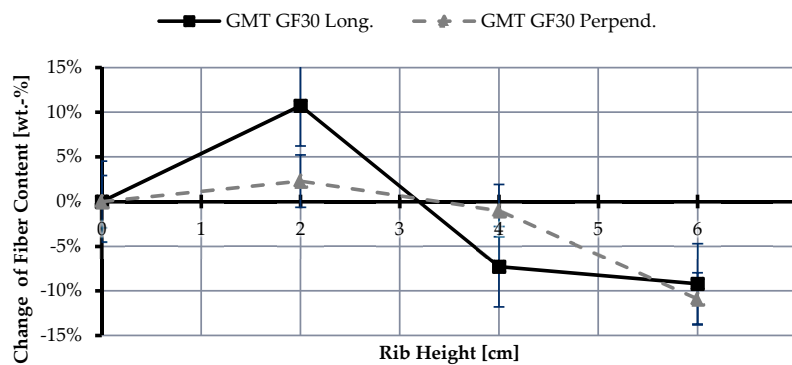
Figure 6. Change of fiber content of GMT GF30 in perpendicular rib.
