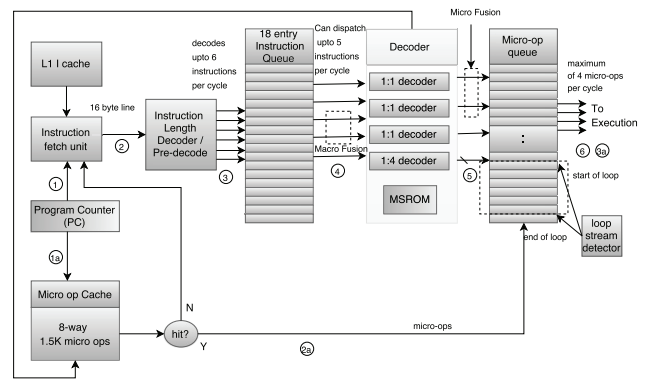
Figure 4. x86 Fetch/Decode Engine
