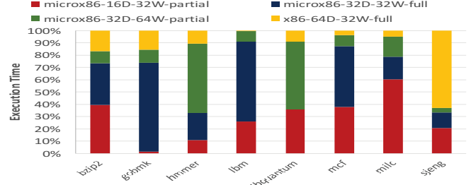
Figure 13. Execution Time Breakdown on the best composite-ISA CMP optimized for Multi-programmed Throughput under 48mm 2 Area Budget most applications migrate to a core with a different feature set at least once. Fourth, the benchmark hmmer that exhibits significant register pressure tends to always execute on a feature set with a register depth of 64. Interestingly, we found that phases with considerable irregular branch activity, due to indirect branches and function pointer calls, prefer full predication since it eases the pressure on the branch predictor by converting some of the control flow into data flow. This is evidenced by the benchmarks sjeng and gobmk .
