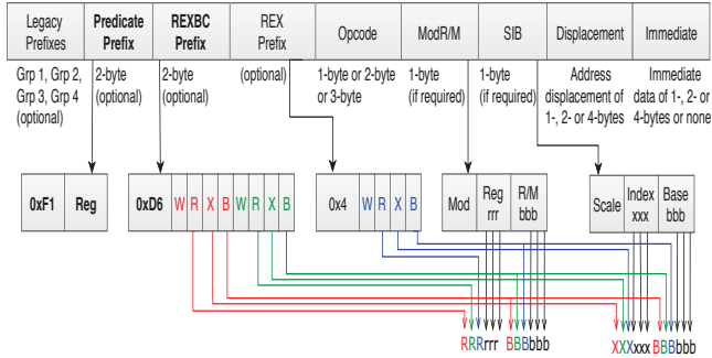
Figure 3. Customizations to x86 Encoding
