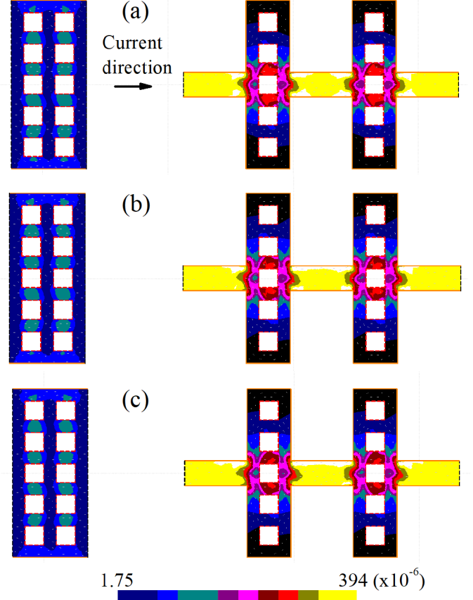
Fig. 5. 3D-MLSI simulation of current distribution of a close packed array and an extended array using the same condition as Fig. 4 with hole dimension reduced to 100 \text{ nm} such that is is much less than \lambda . The color scale indicates a range from 1.75 \times 10^{-6} to 394 \times 10^{-6} .
