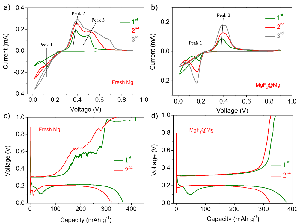
Fig. 3. Cyclic voltammograms using Bi nanorods as positive electrode and different magnesium foils as negative electrodes: (a) Fresh Mg foil and (b) \text{MgF}_2@\text{Mg} foil; Scan rate: 0.1 \text{ mV s}^{-1} . After coating the metal with \text{MgF}_2 , the close voltage difference of the first cycle, \sim 0.2 \text{ V} , between ions-insertion and extraction processes seems to show fast kinetics of migration and diffusion of Mg cation ions. The decomposition of the electrolyte is happening in the voltage above \sim 0.4 \text{ V} in fresh Mg sample and its repeated reaction is observed. Galvanostatic charge-discharge profiles of the 1 st and 2 nd cycle for (c) fresh Mg and (d) \text{MgF}_2@\text{Mg} foil at a current density of 30 \text{ mA g}^{-1} . The electrochemical measurements were carried out at 25^\circ\text{C} in 2025 coin cells. Capacity is calculated based on the weight of the active material mass of Bi.
