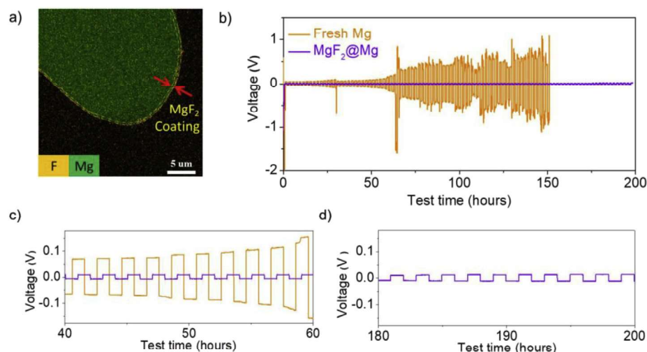
Fig. 2. (a) Cross-section EDS mapping of the as-prepared of the \text{MgF}_2@\text{Mg} electrode. (b) Voltage profiles of the symmetric cells cycling of fresh Mg and \text{MgF}_2 coated Mg at current density of 0.25 \text{ mA cm}^{-2} (1 h for half cycle). (c) and (d) Magnified curves of the cycling for symmetric cells of fresh Mg (orange curve) and \text{MgF}_2@\text{Mg} (violet curve). (For interpretation of the references to color in this figure legend, the reader is referred to the Web version of this article.)
