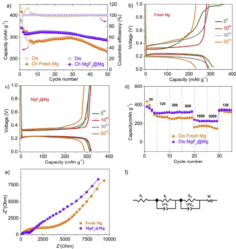
Fig. 4. Charge-discharge tests using Bi nanorods as positive electrode and different magnesium foils as negative electrodes: (a) Cycling performance of fresh Mg and MgF 2 @Mg foil in the range of 0.01-1.0 V, charge-discharge voltage profiles of fresh Mg (b) and MgF 2 @Mg (c) at a current density of 120 mA g -1 between 0.01 and 1.0 V. (d) The comparison of the rate capability of the fresh Mg and MgF 2 @Mg at different current densities. The cells were tested at 30 mA g -1 , 120 mA g -1 , 300 mA g -1 , 600 mA g -1 , 1800 mA g -1 , and 3000 mA g -1 . (e) Electrochemical impedance spectroscopy and fitting results for fresh Mg and MgF 2 @Mg foil after 3 cycles. (f) Equivalent electrical circuit model for the EIS.
