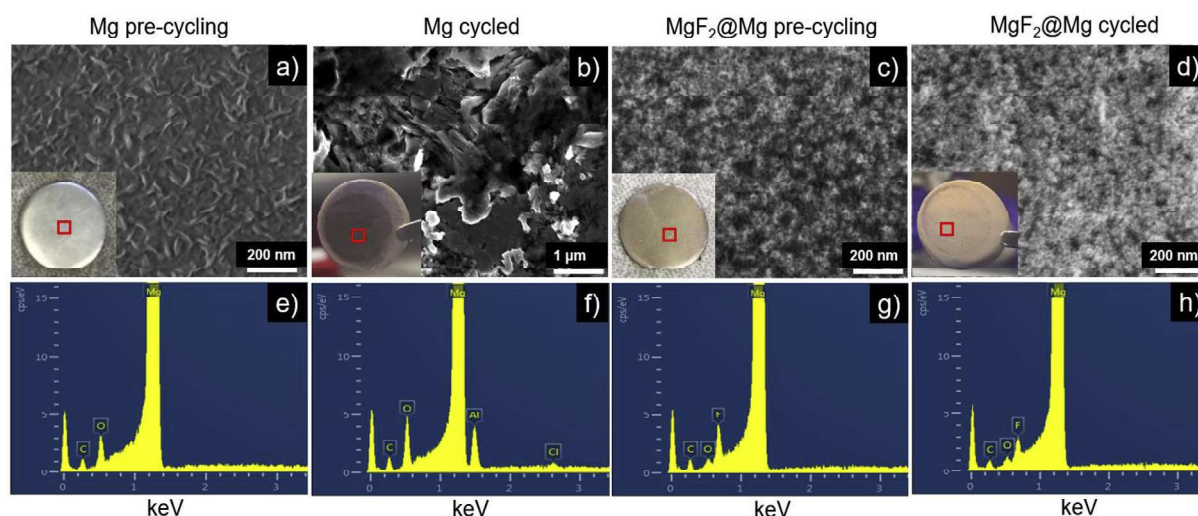
Fig. 5. SEM images of Mg electrodes: fresh Mg before cycling (a) and fresh Mg after 3 cycles (b), \text{MgF}_2 @Mg before cycling (c) and \text{MgF}_2 @Mg after 3 cycles (d). Photographs of the Mg electrodes disassembled from coin cells are shown in the inset. In the fresh sample with \text{MgF}_2 coating, the Mg surface was covered by a nanoparticles sized layer, which is able to prevent the electrolyte decomposition. EDS patterns of the surface of the Mg electrodes: fresh Mg before cycling (e) and fresh Mg after 3 cycles (f), \text{MgF}_2 @Mg before cycling (g) and \text{MgF}_2 @Mg after 3 cycles (h).
