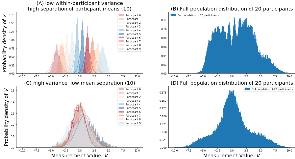
Fig. 4. The variation of a measurement's value has two possible sources. The first is random fluctuations in the value when repeated measurement are taken from an individual (i.e. variation within an individual). The second is random fluctuations in the value when measurements are taken from many individuals through out the population. If the variation within an individual is small compared to the variation among individuals then these measurements may separate participants well. For example, the ten participants in (A) separate well. When the variation condition holds, any measurement value, V_h , from a particular participant h , has a low probability, P_{h'}(V_h) , of coming from another participant h' . For example, repeated CT scans within a small time window of a single individual should have very little variation, however, these scans should be very different between individuals because they measure the entire body. In contrast, when the variation among participants is high compared to the variation among users (C), all measurement values have comparable probabilities of coming from each user (e.g. EEG data has so much noise in the measurement that any individual value can easily have come from many individuals). The population distributions shown in (B) and (D) show the measurement range of the full population of 20 participants. This distribution can tell us if a measurement value is reasonable for a population, that is, has a non-zero probability of being observed. It cannot be used to determine whether the measurements are useful for distinguishing individuals.
