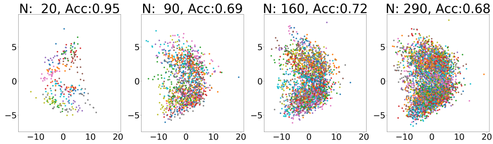
Fig. 6. As we increase the size of the participant count, N , the first two principal components become more crowded. The feature space is often multi-dimensional and these two principal components are the most variable linear combinations of the components in the feature space [18]. The clustering of points in this figure is a two dimensional representation of the per-individual distributions, P_h(V) discussed in Figure 4. This crowding explains why the performance of the identifier will degrade with increased N . When N is large, the various point distributions overlap into an incoherent mass.
