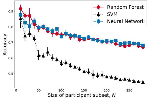
Fig. 8. In the NBA dataset, we can observe a drop in accuracy as the participant count, N , increases regardless of which algorithm was used. For each algorithm, we trained a model with N participants taken from the full population of 290+ players. We then calculated the accuracy for each model and repeated the process for ten iterations. The graph shows the median value and the interquartile range used as error bars. As N increases, we can see that all models' performance degrades. However, some are more impacted than others. As we noted in Section 3.2, each algorithm performs differently when given different types of measurement data. Although these differences indicate that the degradation rates will not be the same, it should be noted that eventually all algorithms degrade when participant count is large enough.
