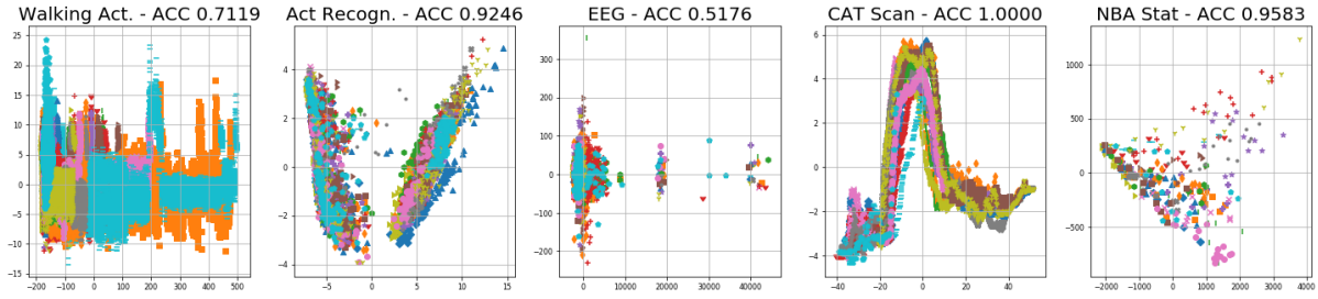
Fig. 9. The first two principal components of the measurements for each dataset is shown. These components can be used to explain the differences in performance observed for each dataset. For the CT scan, activity recognition and NBA stats datasets, the high accuracy is coupled with significant separation in the measurements from each participant. Distinct clusters can be observed indicating that even the limited information captured in these two components is enough to distinguish many participants. The walking activity dataset begins to hint at why performance would degrade as there are clusters, but they fail to be distinct and have some significant overlap. The EEG dataset demonstrates the worst case where there is almost no separation. Most of the participants' measurements are overlapping in one large area with only a small portion lying outside this giant component. All test set measurements from each of the 20 participants that were classified in Figure 3 are plotted. The measurements from each participant have a distinct color and marker shape.
