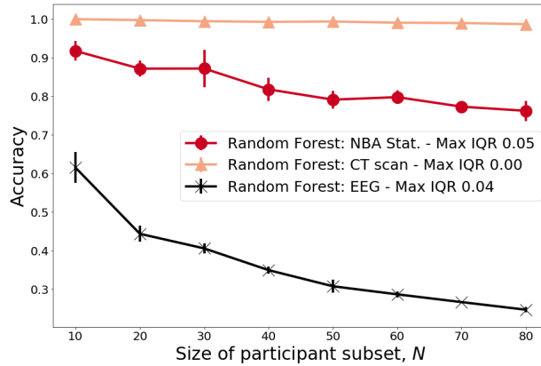
Fig. 5. We can compare the accuracy of the random forest classifier when run on three of the data sets with enough participants to increase N significantly. For each N , we perform 10 runs with randomized subsets of size N . The CT scan dataset has significantly less variation in the performance metric. We measured this by looking at the interquartile range of performance metric values when the given randomized participant subsets. This variation in the CT scan dataset was an order of magnitude lower than the other datasets. The range is not visible in this figure because of scale. Because the CT scan dataset is resilient to variations across humans, its performance degrades much more slowly as the number of participants increases. The variability between randomized subsets may give an indication of how performance will degrade as the participant count increases.
