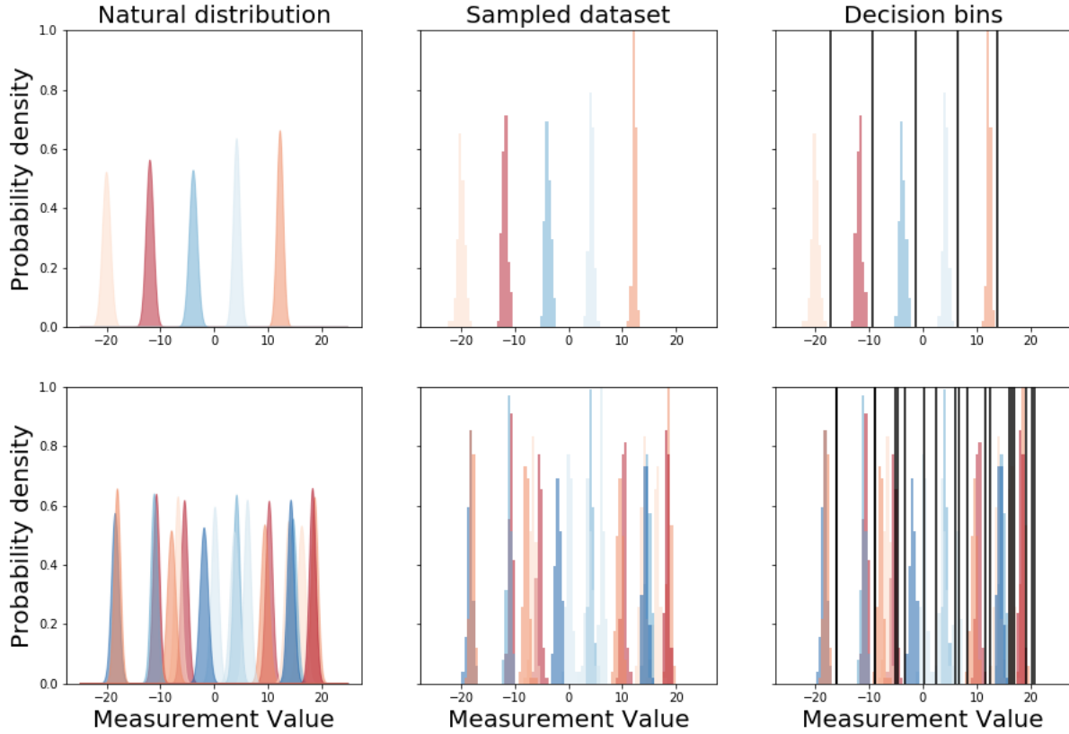
Fig. 7. When the variation within participants is low (low variance in P_h(V) ) and the participant count, N , is small, the probability of observing a measurement value is proportional to the probability of picking that participant, P(V) \propto P(h) . At low N , samples drawn from the natural individual distribution, \mathcal{P}_h(V) , separate well. Thus, it is very easy to draw the boundaries of the bins (e.g. the top row where N = 5 ). As the number of participants increases, the \mathcal{P}_h(V) overlap, thus the samples will overlap, and the bins become more difficult to draw (e.g. the bottom row where N = 20 ). The identification system tries to optimize the placement of bin boundaries by using the sampled dataset as an approximation for the natural distribution.
