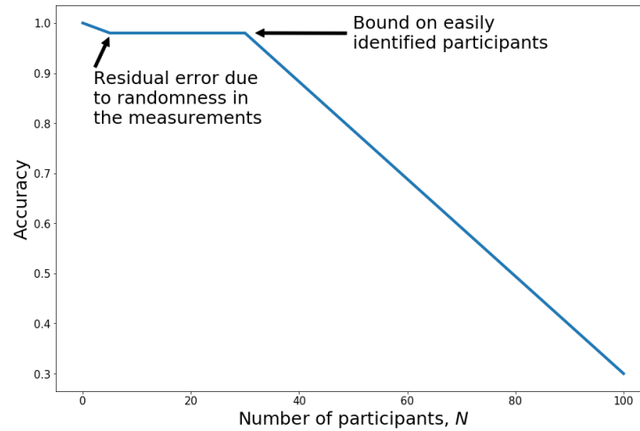
Fig. 1. Even an ideal system that is capable of identifying many users with minimal error will eventually reach an upper bound, N , beyond which the performance will decrease without recovery. Because the measurement value range is finite, the ability to distinguish participants based on these measurements begins to degrade as more participants are added. Consequently, users that were easily identified will be confused with new users that have similar measurement values. We can choose a threshold (e.g. accuracy greater than 80%) below which we declare that the system's error rate makes it unsuitable. Beyond this point, we declare that the system has failed. Because the measurements can vary randomly, it is often very difficult to identify the bound, N , beyond which the performance decreases monotonically.
