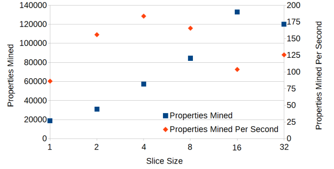
Fig. 3. Slice size affects the mining rate and quantity of output properties.
