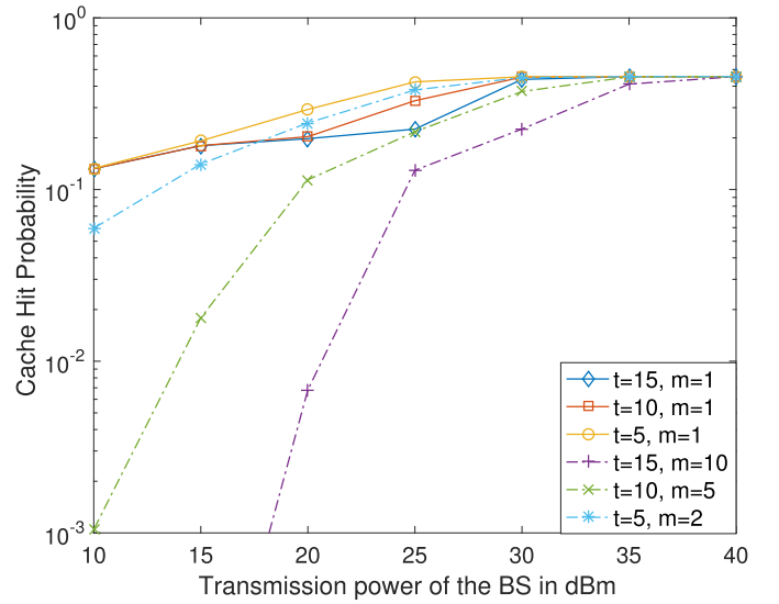
Fig. 7. The impact of the choices of m and t on the cache hit probabilities for the push-then-deliver strategy. N = 20 , \alpha = 3 , R_c = 50m , \lambda_c = \frac{0.01}{\pi R_c^2} , M_s = 3 , t = 5 , m = 1 , and R_l = 1 BPCU, for 1 \leq l \leq 3 . The power allocation coefficient for file f_1 is based on the CR power allocation policy. The power allocation coefficients for files f_2 and f_3 are \beta_2 = \frac{3}{4} and \beta_3 = \frac{1}{4} , respectively. \gamma = 0.5 and |\mathcal{F}| = 3 . Analytical results are used to generate the figure.
