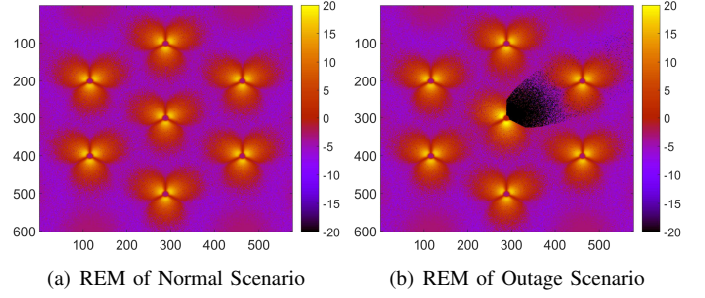
Fig. 1. (a) Radio Environment Map of Normal Scenario (b) Radio Environment Map of Outage Scenario where Antenna Gain of one sector of a BS is attenuated to -50 dBm
