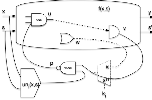
Figure 4: Semi-cycle encryption using unreachable states
