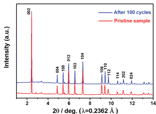
Figure 6. SXRD patterns of a \text{Na}_{0.66}\text{Li}_{0.18}\text{Fe}_{0.12}\text{Mn}_{0.7}\text{O}_2 cathode before and after long-term cycling.
