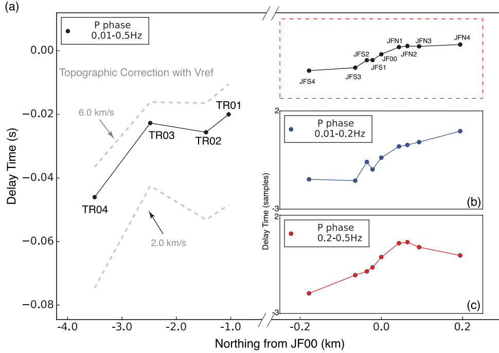
Figure 7. (a) Delay times for teleseismic P phase at 0.01–0.5 Hz. The observed variations in P arrivals are corrected with the traveltime delays due to the geometry of the station and incoming plane wave and topography. The black dots denote delay times derived using 4 \text{ km s}^{-1} reference velocity in topographic correction. The grey dashed lines indicate the lower and higher bound of delay times computed at the TR array using reference velocities of 2 and 6 \text{ km s}^{-1} , respectively. (b) Delay times for teleseismic P phase at 0.01–0.2 Hz. The delay times (blue dots) are shown in the same range outlined by the red dashed box in (a) at the JF array. (c) Same as (b) for 0.2–0.5 Hz.
