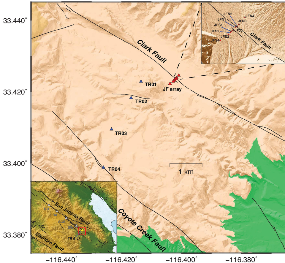
Figure 2. Location map for the JF and TR arrays at the SE end of the Clark fault. The JF array has nine stations separated by \sim 20 – 30 m in the centre with a total aperture of \sim 400 m, and is located on relatively flat topography (top right inset). The TR array to the SW has four stations separated by 0.5 – 1 km, with elevation \sim 100 m higher than the JF array.
