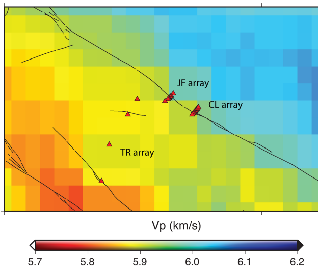
Figure 3. Average P -wave velocity over the depth range 1 – 7 km based on tomographic results of Allam & Ben-Zion (2012). Red triangles indicate stations of the JF and TR arrays, as well as a nearby CL array deployed in 1999.
