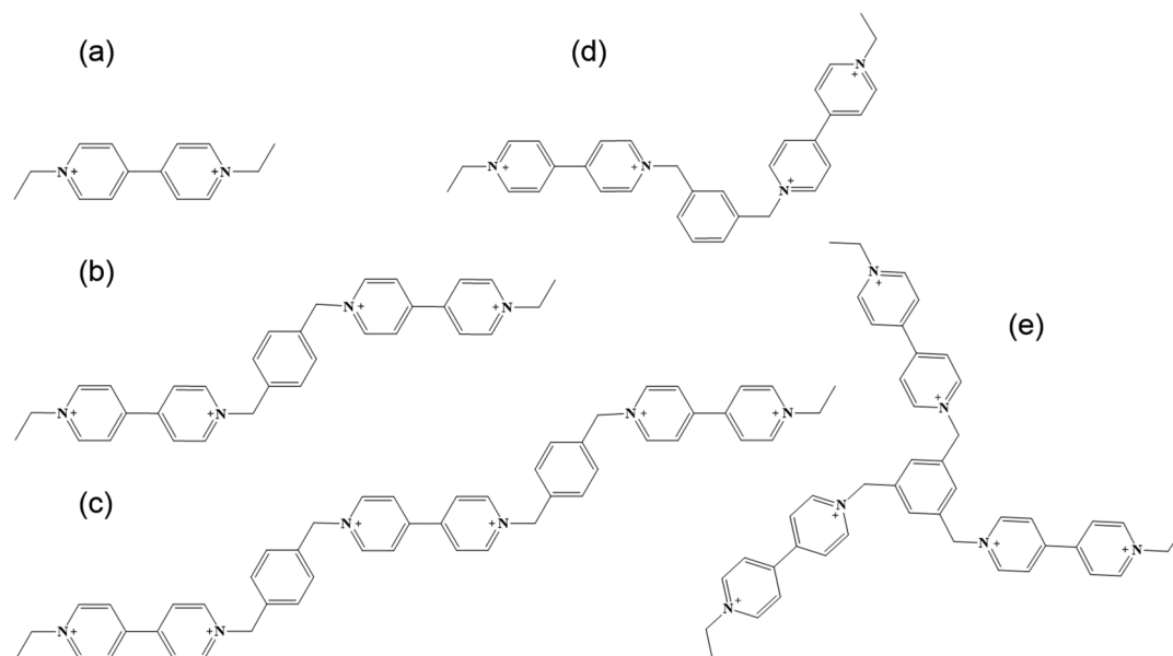
Figure 1. Topology of oligoviologens: (a) monomer; (b) para dimer; (c) linear trimer; (d) meta dimer; (e) star trimer.
