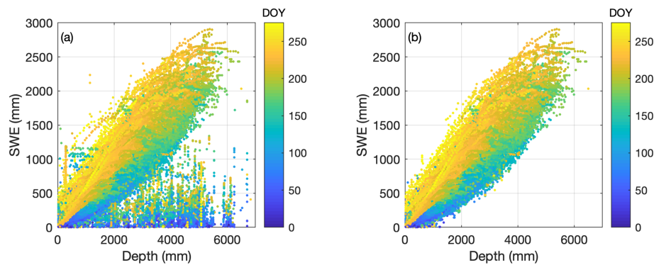
Figure 4. Scatter plot of SWE vs. h for the complete SNOTEL data set before (a) and after (b) removing data points, following the method described in the section Chugach Mountains (Alaska) data. Symbols are colored by day of water year (DOY; 1 October is the origin).
