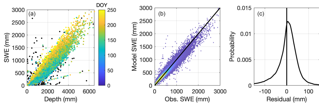
Figure 13. Results from application of the multivariable, two-equation model to the NRCS snow course/aerial marker data set. Panel (a) shows the SWE– h data. Note that the black symbols are points removed during the data preprocessing stage. The remaining symbols are colored by DOY. Panel (b) shows a heat map of the model estimates of SWE against the observations of SWE with the 1 : 1 line included. Warmer colors indicate higher densities of points. Panel (c) shows the probability density function of the model residuals, with the vertical line indicating the mean error, or bias.
