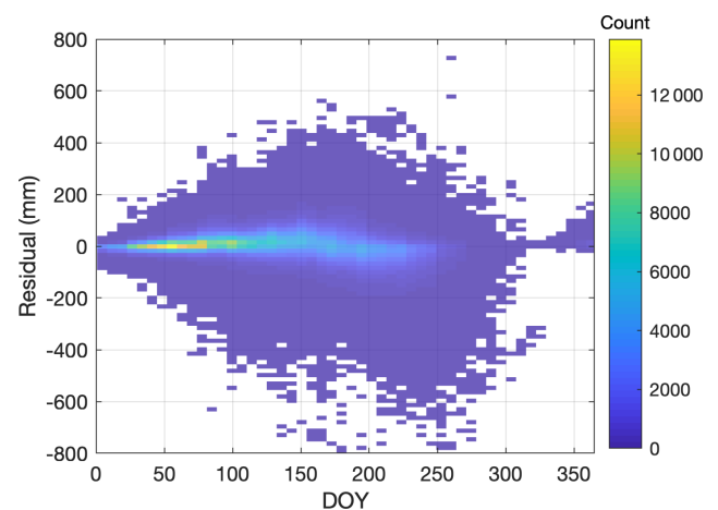
Figure 7. Heat map of SWE residuals as a function of DOY for the application of the multivariable two-equation model to the western North America snow pillow validation data set.
