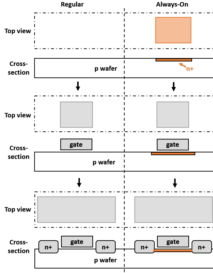
Figure 8: The fabrication of regular (left) and ‘always-on’ transistors (right) by modifying the doping in the channel regions. The mask used for each step is shown in top view, while the sample obtained after each step is shown in cross-section.
