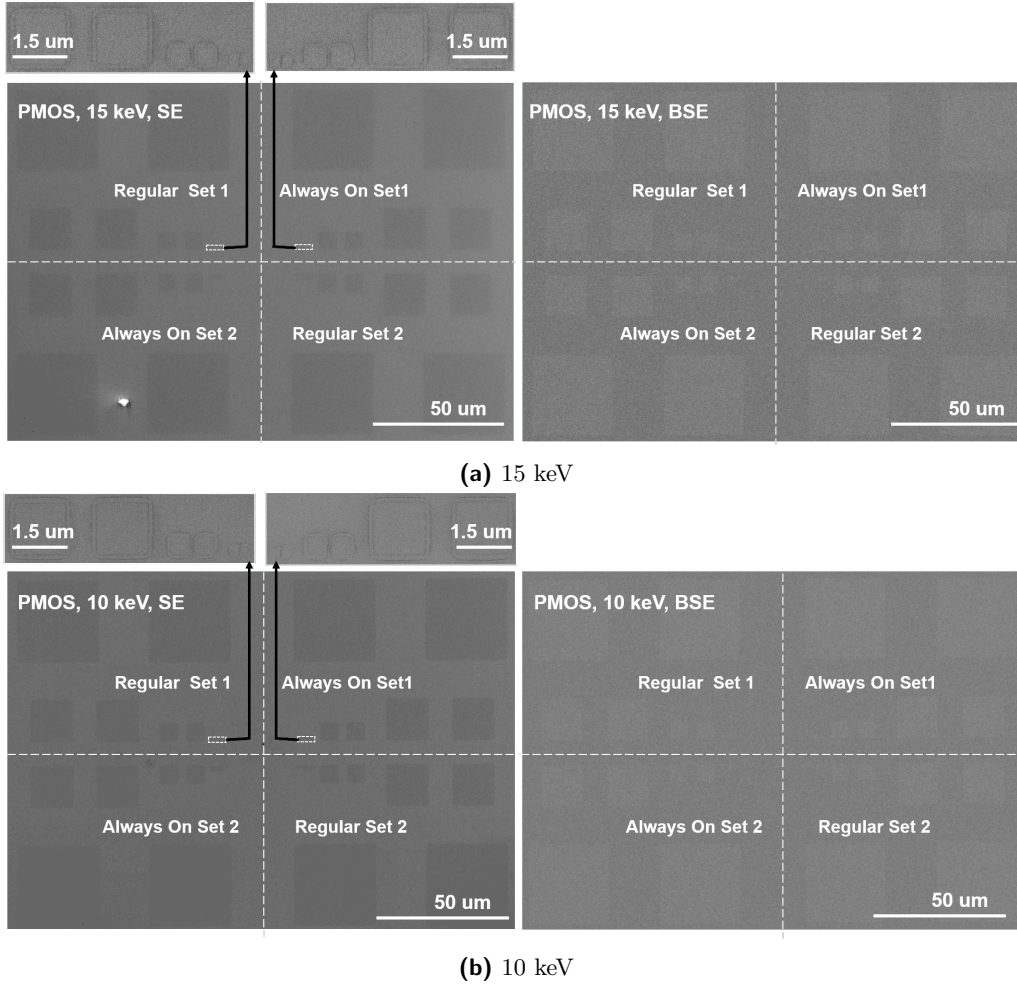
Figure 11: The doped regions of PMOS transistors for regular and ‘always on’ cases are imaged by SE and BSE detectors. The e-beam energy varies from 15 keV to 800 eV. There are 2 sets of transistors with channel lengths varying from 90 nm to 20 \mu\text{m} for each case.
