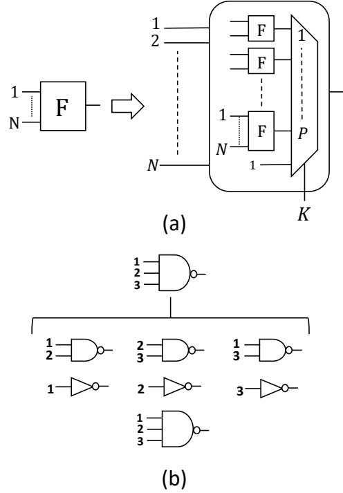
Figure 16: (a) Transforming a camouflaged gate with an unknown number of dummy inputs into a pin permutation network to be solved by SAT. (b) A 3 input NAND gate and its 7 possible candidates.
