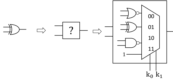
Figure 4: SAT formulation for resolving camouflaged gates. The original gate is unresolvable by imaging ( \rightarrow camouflaged gate). The camouflaged gate is represented by multiple functionalities determined by a key variable ( \rightarrow MUX network controlled by key bits).
