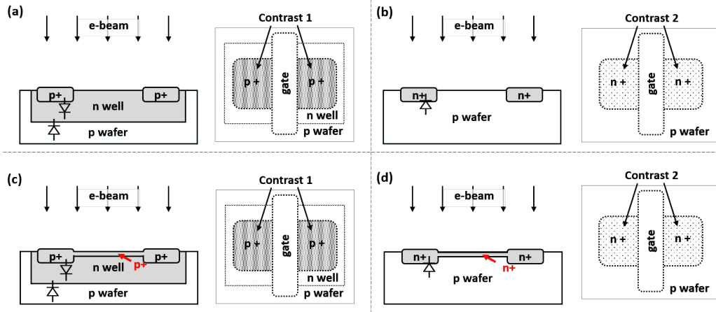
Figure 10: Due to the asymmetry of the p/n interface (indicated by diodes on interfaces), the effective conduction volumes (grayed on the cross-section views) vary between PMOS and NMOS. However, the change between regular PMOS (a) and always-on PMOS (c) is insignificant. The same is the case with regular NMOS (b) and always-on NMOS (d).
