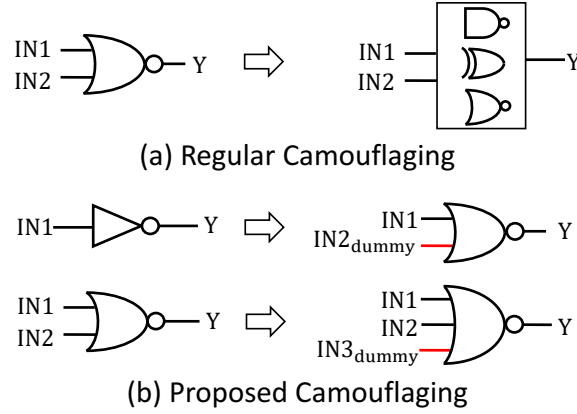
Figure 2: (a) Regular camouflaged gate configurable based on dummy contacts, threshold voltage, or dopant polarity; (b) Proposed camouflaging that introduces dummy inputs.
