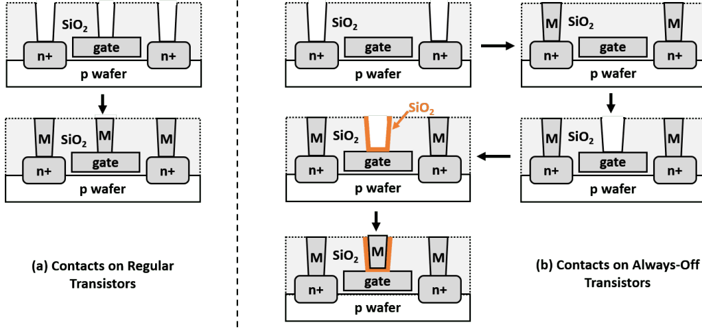
Figure 9: The fabrication of contacts on (a) regular and (b) “always-off” transistors.
