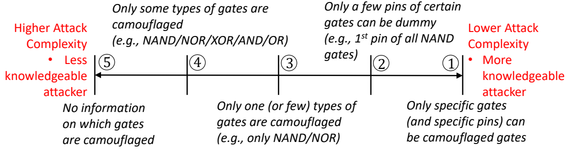
Figure 18: Varying range of available information to the reverse engineer changes de-camouflaging complexity
