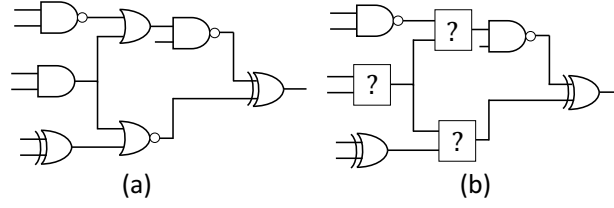
Figure 1: (a) Original gate-level netlist and (b) Netlist containing camouflaged cells obtained after reverse engineering.
