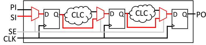
Figure 3: Scan chain-inserted design where PI, SI, SE, CLK, CLC, and PO stand for Primary Inputs, Scan In, Scan Enable, Clock, Combinational Logic Cone and Primary Outputs.
