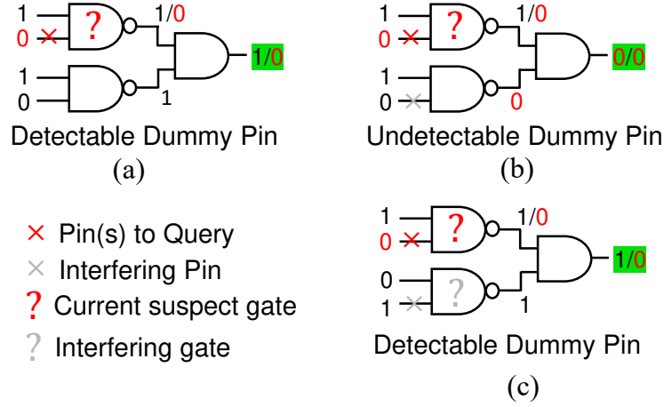
Figure 17: (a) A detectable dummy pin which can be sensitized and propagated to output. (b) Undetectable dummy pin whose output is contaminated by another dummy pin. (c) Detecting dummy pin in the presence of an interfering dummy pin.
