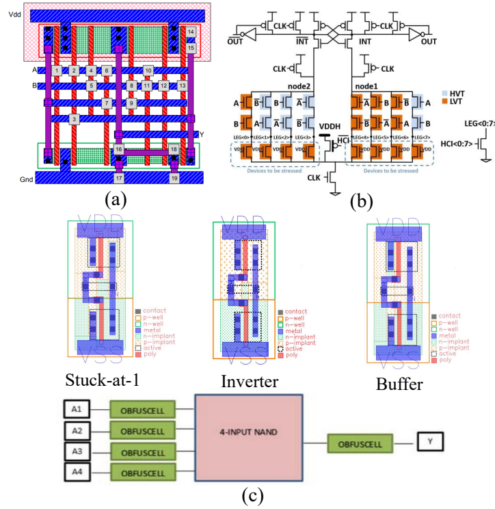
Figure 5: (a) Dummy contact-based camouflaged gate that can be configured as NAND , NOR or XOR [RSSK13] (b) Post-manufacturing programmed threshold voltage defined gate [AEM18] (c) Camouflaged gate based on dopant polarity - The ‘obfuscell’ can be configured as an inverter, buffer or be stuck-at-1/0. The cell is combined with a logic gate to create a multifunctional ‘ObfusGate’ [MBPB15]
