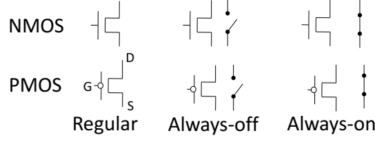
Figure 6: Regular NMOS/PMOS transistors and always-on/always-off transistors (where S \rightarrow Source, G \rightarrow Gate, D \rightarrow Drain).
