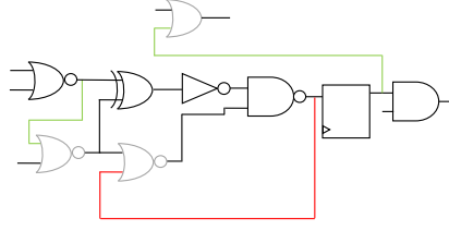
Figure 15: Valid nets (marked in green) for the dummy inputs of the covert gates. Invalid nets are shown in red. Note that sequential feedback loops are valid, as loops are common in sequential circuits with state.
