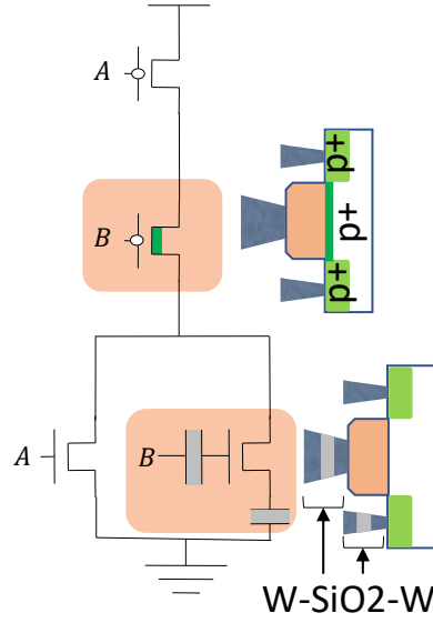
Figure 14: Modeling the always-on transistor (above) and always-off transistor (below). W represents the tungsten metal contact, p+ is the heavily doped diffusion region and \text{SiO}_2 is the insulating layer on the gate and source terminals, modeled by a parallel plate capacitor.
