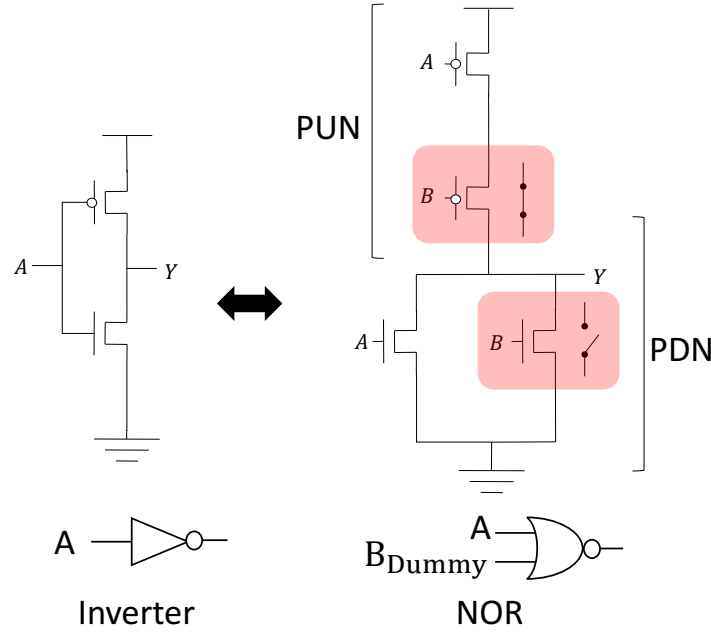
Figure 7: A 2 input NOR gate where B is a dummy input. PMOS transistor in the pull-up network (PUN) connected to B is always on (short circuit) and the NMOS transistor in the pull-down network (PDN) connected to B is always off (open circuit). As a result, the gate behaves like an inverter with input A .
