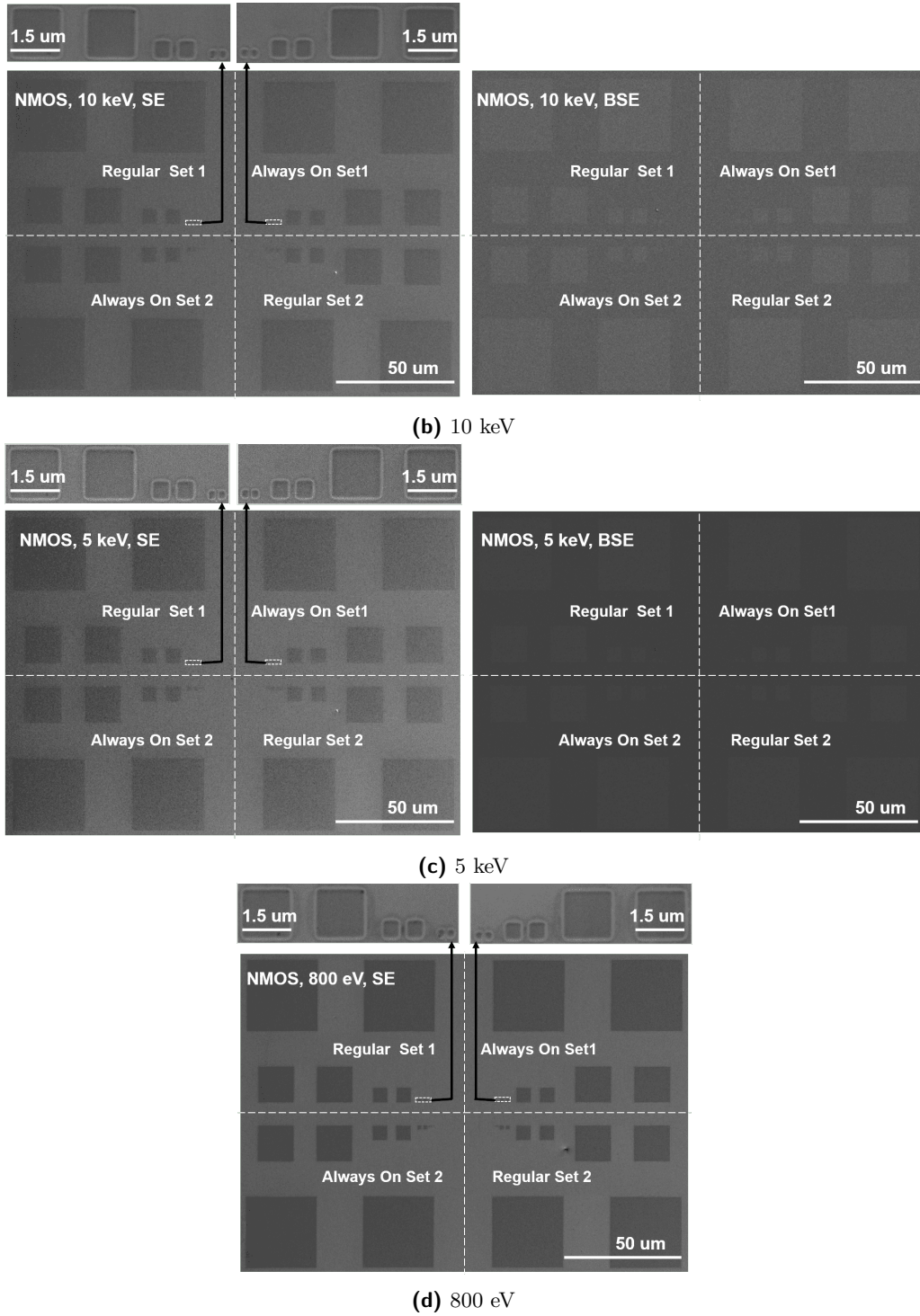
Figure 12: The doped regions of NMOS transistors for regular and 'always on' cases are imaged by SE and BSE detectors. The e-beam energy varies from 15 keV to 800 eV. There are 2 sets of transistors with channel lengths varying from 90 nm to 20 \mu\text{m} for each case. (continued..)
