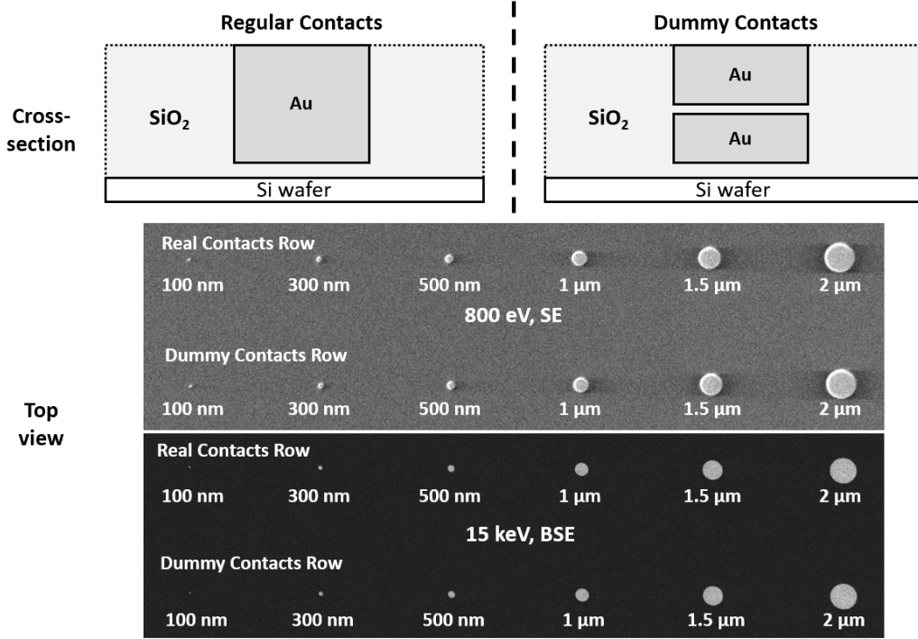
Figure 13: Contacts and dummy contacts for regular and ‘always-off’ transistors under SE and BSE imaging conditions.
