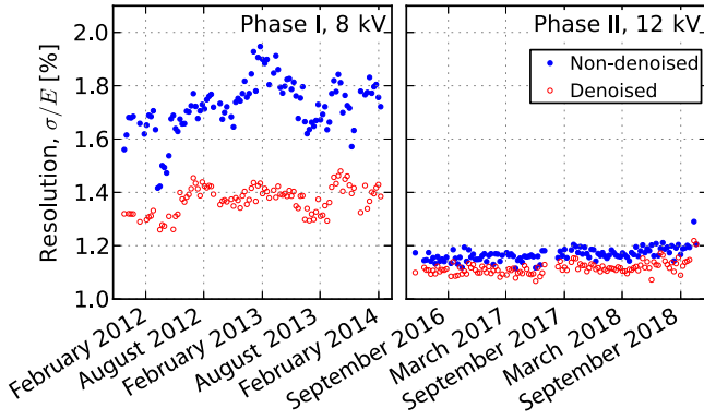
FIG. 2. Energy resolution of SS events measured using a ^{228}\text{Th} calibration source deployed to a position near the cathode. The effect of the denoising algorithm and weekly variation of the resolution at the 2615 keV ^{208}\text{Tl} \gamma line are shown for both Phase I and Phase II. The resolution worsened slightly after a xenon recovery in July 2017 due to a power outage. A degraded resolution due to an increase of excess noise is visible in the last weeks of Phase II.
