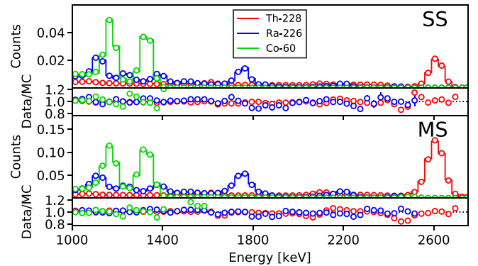
FIG. 1. Comparison of energy distributions in data (circles) and MC (lines) for SS (top half) and MS (bottom half) events from calibration sources positioned near the cathode.
