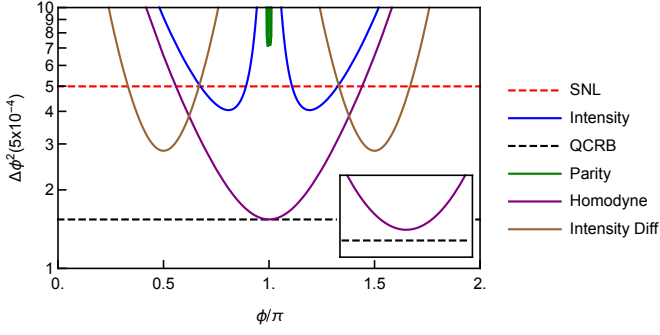
FIG. 2: Log plot of phase variance for various detection schemes for a coherent state and squeezed vacuum into an MZI, as a function of the unknown phase difference \phi . Loss parameters have been set to L = 20\% . Input state parameters for each respective state are set to |\alpha|^2 = 500 and r = 1 . SNL and QCRB are also plotted with the same loss parameters. Note that a homodyne measurement nearly, but not exactly, reaches the QCRB as shown by the inset.
