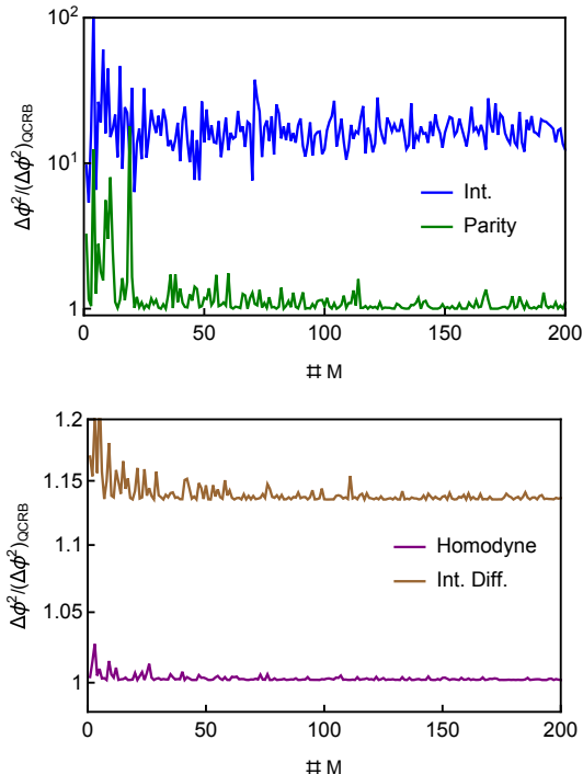
FIG. 4: Log plots of phase variance ratio to the lossless QCRB as a function of number of measurements ( M ) under phase drift noise only. For all plots shown, |\alpha|^2 = 100 , r = 1 and the standard deviation of the chosen Gaussian distribution is fixed to \sigma = 0.15 . Note that parity and intensity measurement remain noisy even after 200 averaged measurements, where homodyne and intensity difference approach their optimal phase variance quickly in M .
