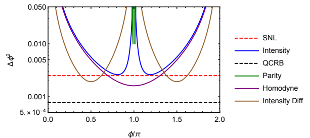
FIG. 5: Log plot of phase variance of the various detection schemes, with introduction of thermal photon noise into both interferometer arms, of total average photon number of n_{\text{th}} = 1 . Strength of the two input sources are set to |\alpha|^2 = 500 , r = 1 . Note that homodyne loses most of its previous advantage over intensity difference but remains the superior measurement choice.
