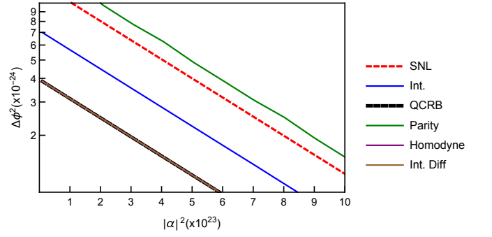
FIG. 3: Log plot of phase variance for various detection schemes for a coherent state and squeezed vacuum into an MZI, as a function of the average coherent photon number, |\alpha|^2 , shown in the very large power regime. Total loss parameters have been set to L = 20\% . We have assumed one can set the control phase to its optimal value, to obtain the best phase variance in each measurement choice. Squeezing strength in the squeezed state is set to r = 1 . Note that Parity is now not able to achieve even sub-SNL, due to loss, while homodyne and intensity difference quickly approach the QCRB (appear on top of one another). SNL and QCRB are also plotted with the same lossy parameters.
