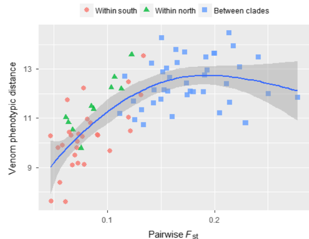
Fig. 5 Relationship between pairwise F_{ST} of rattlesnake populations and pairwise distance between the same populations in Euclidean distance in cl-transformed venom phenotype space. Comparisons are within the southern clade (red), northern clade (green) or between clades (blue).
