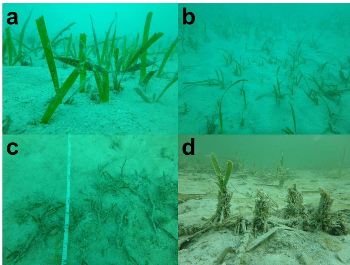
Fig. 3 Photos of moderate (5–10 cm) T. testudinum seagrass burial after Hurricane Irma at FKNMS site 255 ( a ) and site 239 ( b ). Note how sediments separate leaves of the same short shoot, and ligules (leaf bases) are buried below a layer of sediment. Photo of strong seagrass erosion of T. testudinum after Hurricane Irma at FKNMS site 276 ( c ).
