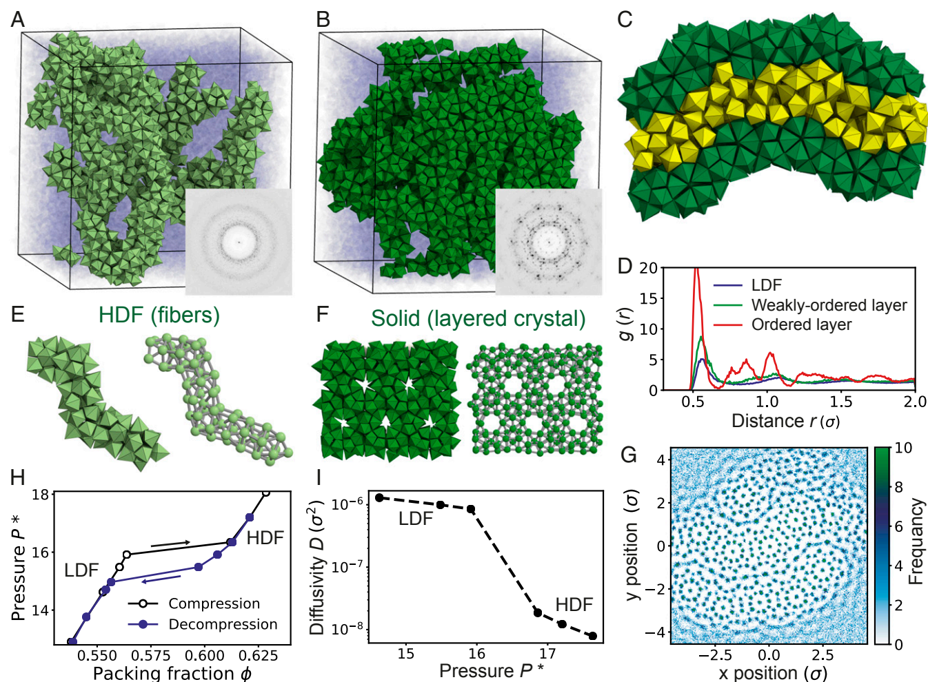
Fig. 4. Crystallization of a layered crystal (oF244) via fiber formation. Hard pentagonal bipyramids (PBPs) self-assemble into a layered crystal (oF244) at constant packing density \phi = 0.580 . (A) In the early stage of crystallization, hard PBPs separate into an LDF (transparent blue) and an HDF that consists of fiber-like motifs (light green). (B) The obtained crystal consists of layers of parallel fibers (dark green). (C) A cross-section of the crystal phase shows that a crystal layer (dark green) and a weakly ordered layer (yellow) alternate within the crystal. (D) The radial distribution function g(r) of the crystal layers, the weakly ordered layers, and the LDF. (E) A fiber-type prenucleation motif (Left) found in the HDF. (Right) Centers of PBPs and bonds (gray). (F) Part of a crystal layer with PBP representation (Left) and its centers (Right). (G) A density plot of particle centers for a cross-section of the crystal averaged over 200 \times 10^6 Monte Carlo sweeps. See Movie S3 for the movement of particles in each layer. (H) Equation of state of hard PBPs. Each data point is obtained by a single isobaric Monte Carlo run initialized in a disordered starting configuration for compression (black line) and initialized in an HDF configuration for decompression (blue line). (I) Diffusivity of the 2 fluids near the LDF-to-HDF transition.
