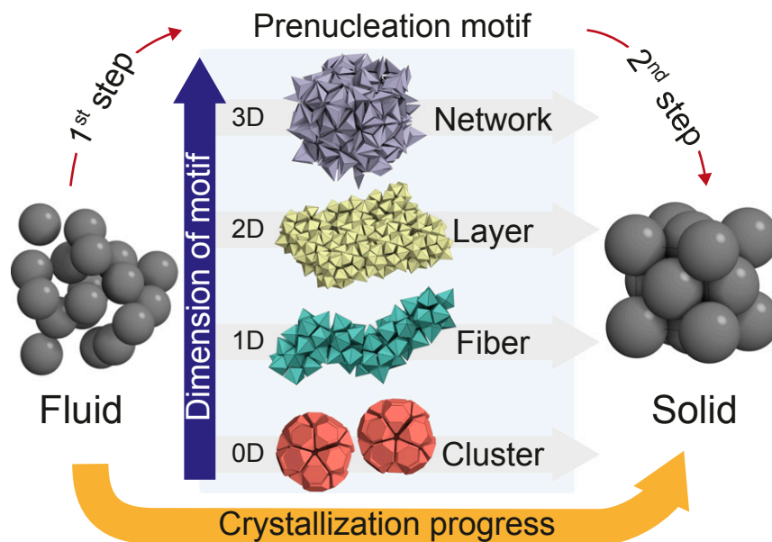
Fig. 1. Categorization of 2-step nucleation pathways. Two-step nucleation pathways are mediated by precursors that can be categorized by the dimension of the prenucleation motif. We distinguish in our simulations of 3 different systems clusters (zero-dimensional motif), fibers (one-dimensional) and layers (2D), and networks (3D), respectively. The dimension of the motif is a direct consequence of geometrical frustration that builds up as prenucleation motifs grow (27).
