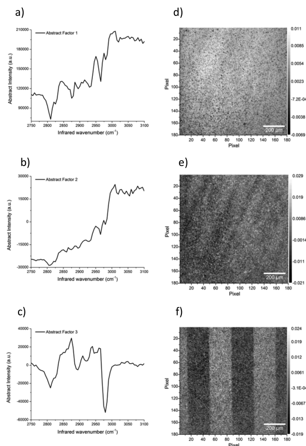
Figure 7. First three abstract factors from row matrix (a–c) and column matrix (d–f) obtained by PFA of 500 shot ODT-MeOHT sample data matrix.
