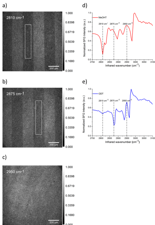
Figure 1. ODT-MeOHT sample SFG images at (a) 2810 cm -1 , (b) 2875 cm -1 , (c) 2950 cm -1 , (d) MeOHT SFG spectrum, and (e) SFG spectrum of ODT stamped region.
