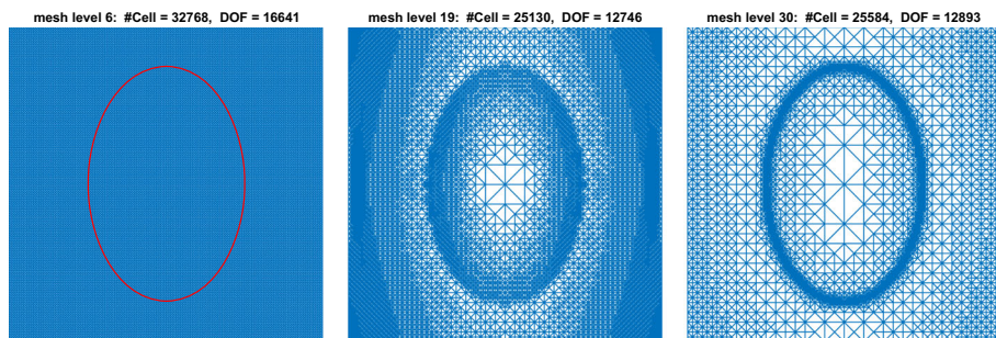
Fig. 3 Uniform mesh for IFEM (left), adaptive mesh for IFEM (center), adaptive mesh for FEM [13] (right) for Example 6.1
