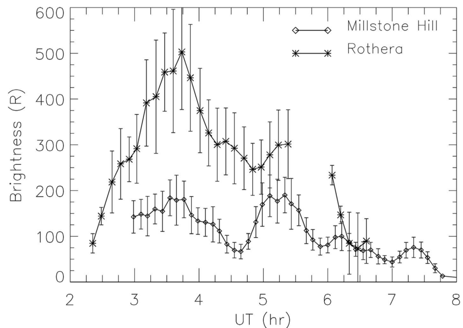
Figure 6. Millstone Hill (diamonds) and Rothera (asterisks) stable auroral red arc brightness. The stable auroral red arc curves at both sites follow a similar trend, with Rothera being larger than Millstone Hill. The error bars represent the uncertainty in the determination of the brightness values. The small gap in the Rothera curve is due to clouds that affected the fitting process.
