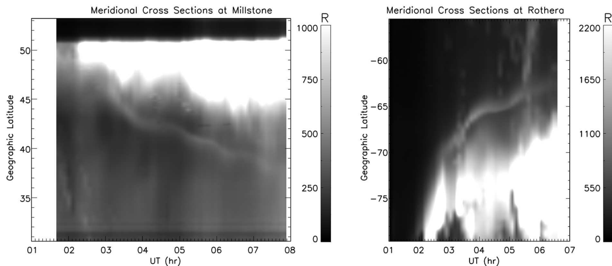
Figure 7. (left) Meridional cuts 10-pixel-wide from Millstone Hill. The bright structures on the top are auroral signatures. The stable auroral red arc appears around 0300 UT at \sim 47^\circ geographic latitude. (right) Meridional cuts 10-pixel-wide from Rothera. The stable auroral red arc is observed before 0300 UT.
