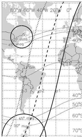
Figure 10. Defense Meteorological Satellite Program (DMSP) F15 passes on 1 June 2013. The first pass (p1, thick solid line) crossed 50° mag latitude at 0° longitude at 0400UT; the second pass (p2, dashed thick line) at ~25°W at 0600UT; the third pass (p3, dotted line) at ~55°W at 0730UT. Circles represent 160° field-of-view of the all-sky imagers. Map is shown using a Mercator projection. Stable auroral red arc signatures are observed inside 45–50° and -45–50° magnetic latitudes.
