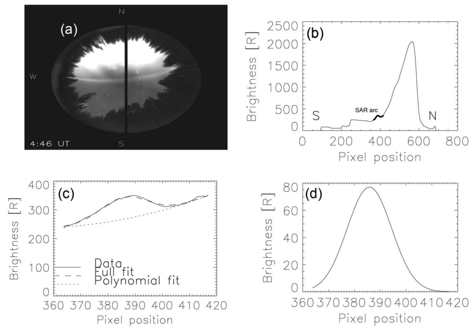
Figure 5. (a) Unwarped and calibrated Millstone Hill image at 0446 UT. The black line represents a north-south 10-pixel-wide meridian cut. (b) Average cut covering the entire image. The pixel positions in the horizontal axis can be uniquely related to geographic latitudes. The thick superposed curve represents the subrange of data that will be fitted to obtain stable auroral red arc parameters. (c) Stable auroral red arc data obtained from the average cut (solid line), full fit (dashed line), and polynomial fit (dotted line). (d) Resulting Gaussian fit obtained by subtracting the full and polynomial fits shown to the left. From this curve the brightness, location, and width of the arc can be obtained.
