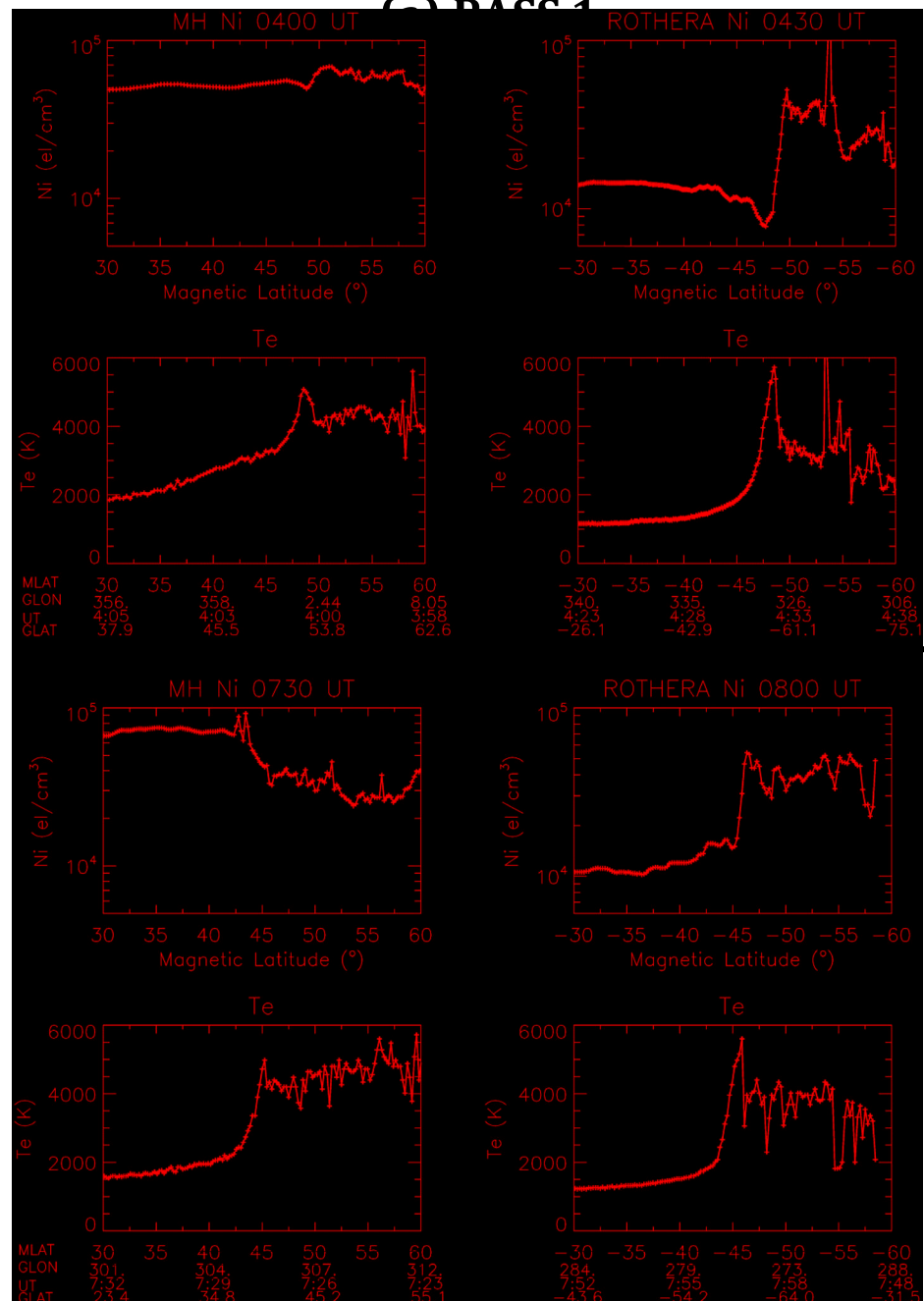
Figure 11. (a) PASS1: Defense Meteorological Satellite Program (DMSP) F15 observations of (top panels) total ion density N_i and (bottom panels) electron temperature T_e (left) in the northern hemisphere at ~0400UT and (right) in the southern hemisphere at ~0430UT. The typical signatures of a stable auroral red arc (low N_i , high T_e ) are observed at subauroral magnetic latitudes ~50°, similar to the arcs locations. (b) PASS 3: similar to (a) but at 0730 UT in the northern hemisphere and ~0800 UT in the southern hemisphere. Stable auroral red arc signatures are observed at lower latitudes, around 45° magnetic latitude, in agreement with the all-sky imager observations at Millstone Hill (the Rothera all-sky imagers had stopped taking data at 0700UT).
