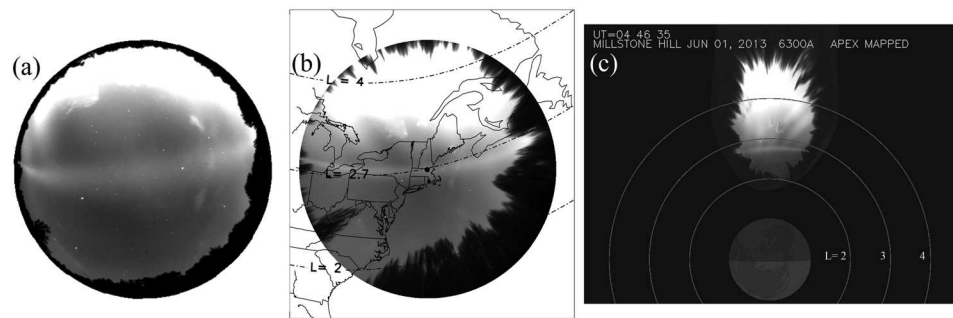
Figure 3. All-sky image in 630.0 nm that shows a stable auroral red arc and the diffuse aurora in (a) raw data format and (b) “unwarped” upon a geographic map for an assumed emission altitude of 400 km. Trees at low-elevation angles restrict useable data to \sim 160^\circ field of view. Lines with constant L-shell values are shown for L=2 , L=2.7 , and L=4 ; (c) mapped into the geomagnetic equatorial plane. L values of 2, 3, and 4 are shown.
