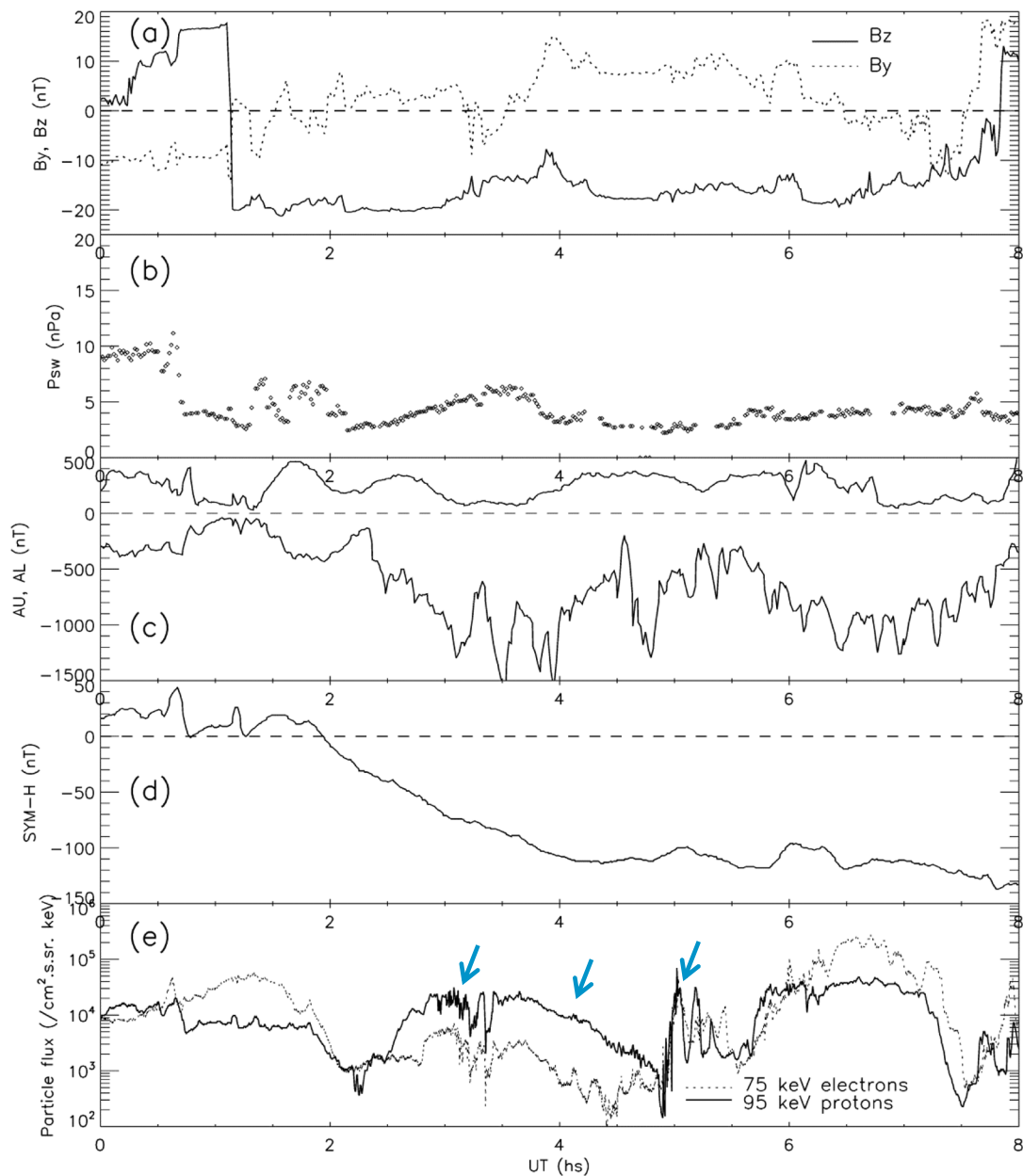
Figure 12. (a) Solar wind B_y and B_z components. (b) Solar wind pressure. (c) Auroral AU and AL indices. (d) Equatorial SYM-H index. (e) Particle flux from GOES-15. Arrows indicate the times when the brightness and speeds of the arcs change.
