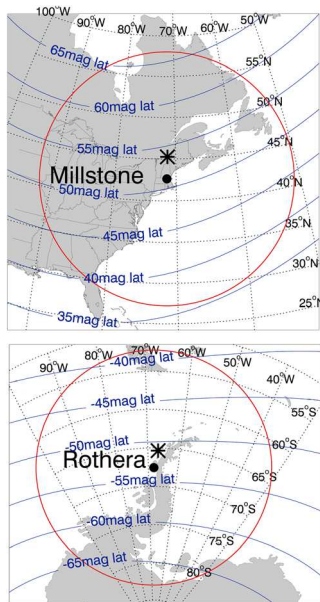
Figure 2. (top) Field-of-view of the Millstone Hill all-sky imager for zenith angles <85^\circ and emission height at 400 km; (bottom) field-of-view of Rothera's all-sky imager. The solid black circles refer to zenith at each location, and the asterisks represent their geomagnetic conjugate points.
