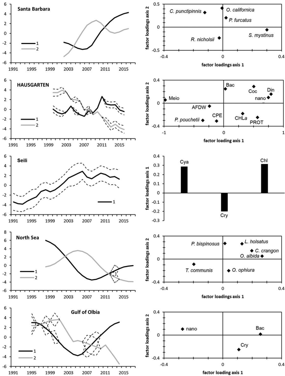
Figure 3. Common trends (left) and corresponding factor loadings (right) for the five LTER sites obtained by means of DFA. Only factor loadings above the cut-off of 0.2 in absolute value are shown. Common trends and factor loadings are untitled. Dashed line in graphs indicates the confidence interval of the DFA model. Bac = Bacillariophyceae, Chl = Chlorophyceae/Chlorophyta, Coc = Coccolithophyceae, Cry = Cryptophyceae, Cya = Cyanophyceae, Din = Dinophyceae, nano = nanoplankton/nanoflagellates, Ppou = Phaeocystis pouchetii , CHLa = chlorophyll a , AFDW = organic matter in the sediments as ash-free dry weight, CPE = sediment-bound chloroplastic pigments, PROT = particulate proteins in the sediments, Meio = meiofauna.
