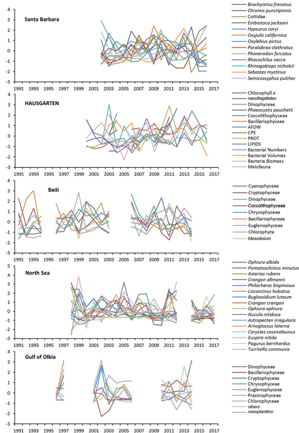
Figure 2. Transformed and standardized time-series at the various LTER sites. AFDW = organic matter in the sediments as ash-free dry weight, CPE = sediment-bound chloroplastic pigments, PROT = particulate proteins in the sediments.
