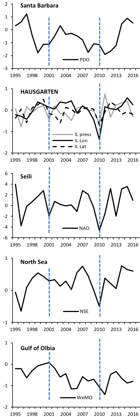
Figure 4. Multiannual yearly mean variability of the different climate indices (PDO, IL, NAO, NSE, WeMO) considered in the study. The blue dotted lines indicated the Climate Regime Shifts (CRS).
