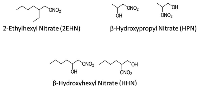
Fig. 1 Structures of the gas phase organic nitrates used in this study. The synthesis of the hydroxynitrates resulted in the presence of the two isomers.
