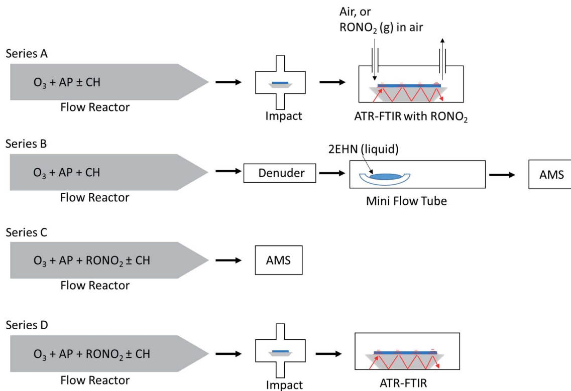
Fig. 2 Schematic of the four experiment types. In Series A, SOA particles are formed in the absence of organic nitrates ( RONO_2 ) in the stainless steel flow reactor and impacted on an ATR crystal to generate a thin film of particles, over which RONO_2 at near saturation vapor pressures ( 4.7 \times 10^{15} (2EHN), 3.9 \times 10^{15} (HPN) and 1.7 \times 10^{14} (HHN) molecules per cm^3 ) were flowed and the uptake of RONO_2 was measured by ATR-FTIR. In Series B, SOA particles were generated in the stainless steel flow reactor and then passed through a charcoal denuder before subsequently being flowed into a 1 m long glass flow tube and exposed to 2EHN through either a reservoir with a pure liquid or a trap flowing air over the pure liquid, and analyzed by HR-ToF-AMS. In Series C, RONO_2 at lower levels ( 1.4 \times 10^{14} (2EHN), 1.2 \times 10^{14} (HPN) and 5.0 \times 10^{12} (HHN) molecules per cm^3 ) were incorporated into SOA particles as they form and grow in the stainless steel flow reactor. These particles were quantified by HR-ToF-AMS. In Series D, the same particles as in Series C were impacted on an ATR crystal and partition coefficients were determined from the quantification of RONO_2 by ATR-FTIR. For Series A, the gas-phase organic nitrate concentration was measured using GC-MS from the trap. For Series B, the gas-phase 2EHN concentration was measured directly from the mini flow tube. For Series C/D, the gas-phase organic nitrate concentration is calculated from the measured concentration exiting the trap and accounting for dilution (a factor of 34).
