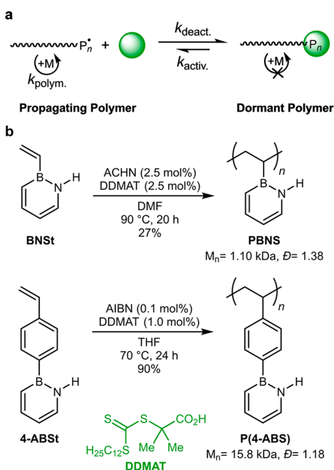
Scheme 3. (a) Controlled Radical Polymerization by Reversible Deactivation. a (b) Liu and Jäkle: RAFT Polymerization of BNSt and 4-ABSt. 28, b
