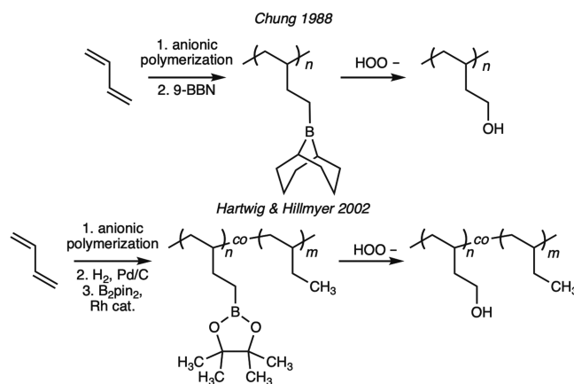
Scheme 4. Borane Strategy for Polyalcohol Synthesis
