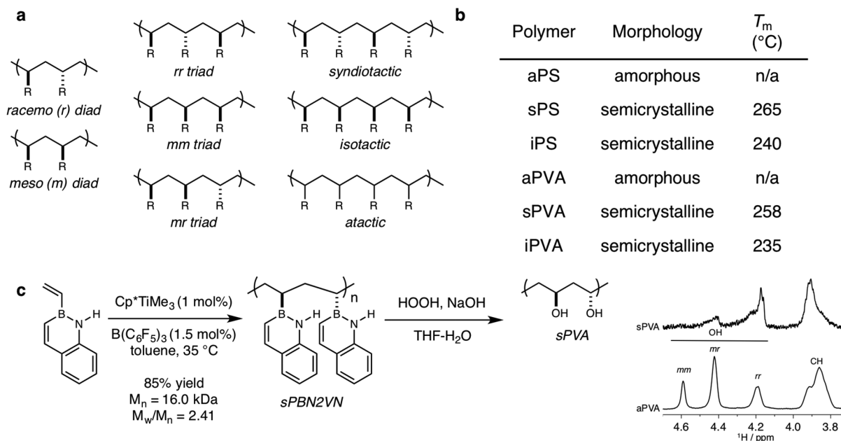
Scheme 6. (a) Stereoregular Polymer Nomenclature. (b) Variation in Physical Properties with Tacticity. (c) Klausen: Synthesis of Syndiotactic PBN2VN by Coordination–insertion Polymerization a
