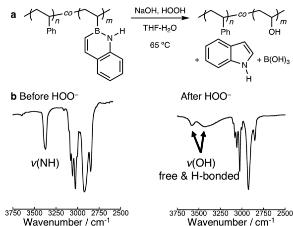
Scheme 5. Klausen: Postfunctionalization of BN2VN Copolymers. (a) Typical Reaction Conditions for Oxidation of PBN2VN- co -PS to PVA- co -PS. (b) Cropped IR Spectra Highlighting the Disappearance of BN2VN \nu(\text{NH}) Feature and Appearance of PVA \nu(\text{OH}) Features after Oxidation a
