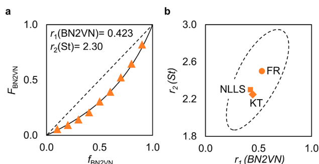
Figure 2. Klausen: styrene–BN2VN reactivity ratios. (a) Mayo–Lewis plot for the statistical copolymerization of BN2VN and styrene with AIBN. 32 Dashed line represents a random copolymerization ( r_1 = r_2 = 1 ); solid curve is a fit to the experimental data and indicates a statistical copolymerization where r_1 = 0.423 and r_2 = 2.30 . F_{\text{BN2VN}} = fractional composition of BN2VN in the copolymer; f_{\text{BN2VN}} = fractional composition of BN2VN in the monomer feed. (b) Reactivity ratios of statistical copolymerization of BN2VN and styrene with AIBN by Fineman–Ross (FR), Kelen–Tüdös (KT), and nonlinear least-squares (NLLS) analysis. Dashed ellipsoid represents the 95% confidence interval of NLLS analysis. 32
