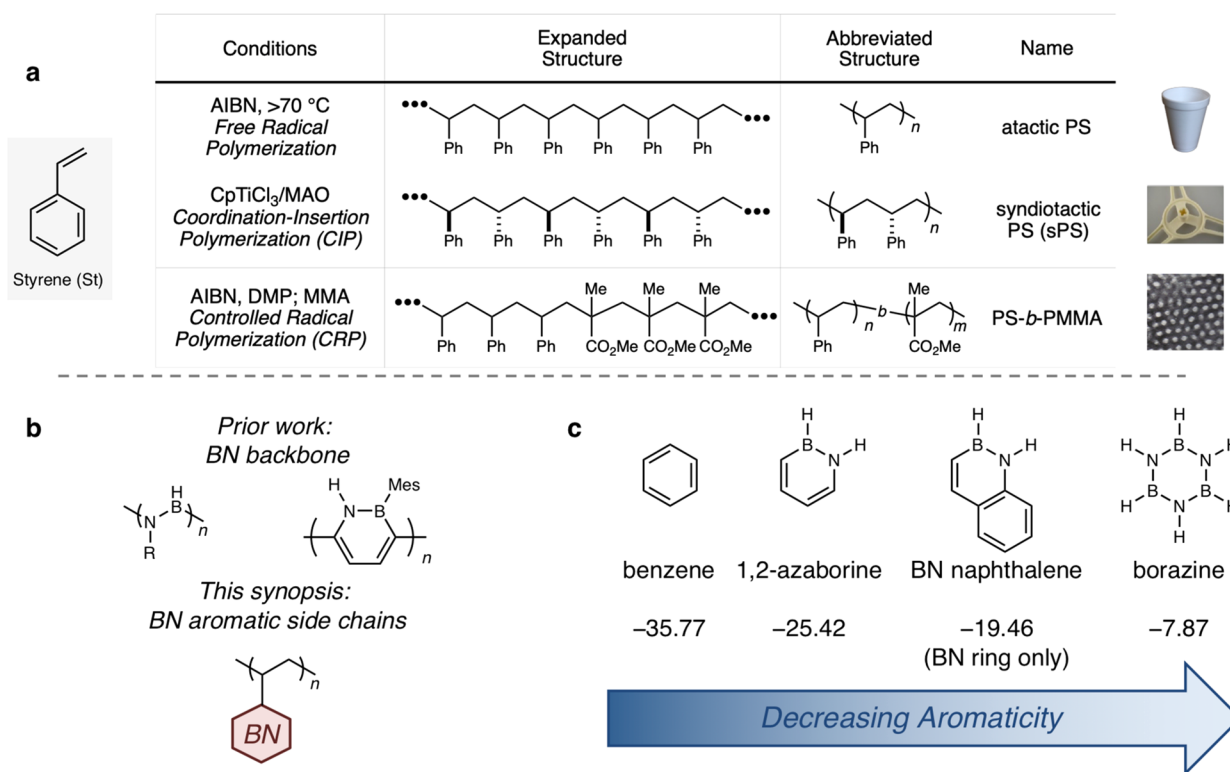
Figure 1. (a) Styrene polymerization and applications. (b) Prior work in BN for CC isosterism in polymeric materials. (c) BN aromaticity. NICS(0) xyz (ppm) values excerpted from Baranac–Stojanović et al. 23,24
