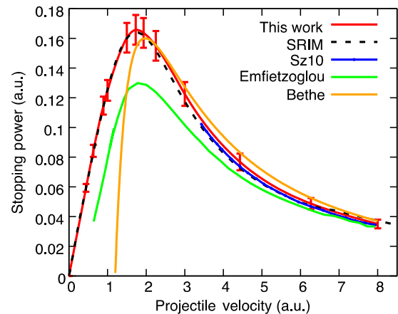
FIG. 1. Electronic stopping power curve from our first-principles simulation in comparison to the experimental data by Shimizu and co-workers [40,41] (Sz10), the SRIM [16] model, the Bethe model [44] with I = 78 \text{ eV} recommended by the International Commission on Radiation Units and Measurement [8], and Emfietzoglou’s model [10–12].
