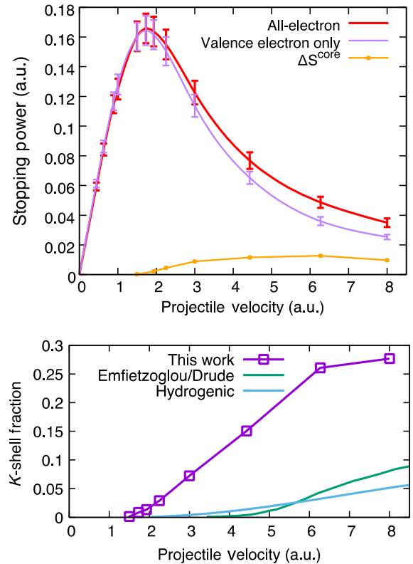
FIG. 2. (Top panel) Contribution of the K -shell (oxygen 1s electrons) excitation to electronic stopping power curve, \Delta S^{\text{core}} , calculated as the difference between the all-electron and the valence-electron-only results. (Bottom panel) The fraction of the K -shell contribution to the stopping power, in comparison to the Emfietzoglou or Drude model [11,12], and the hydrogenic generalized oscillator strength model [11,49,52,53].
